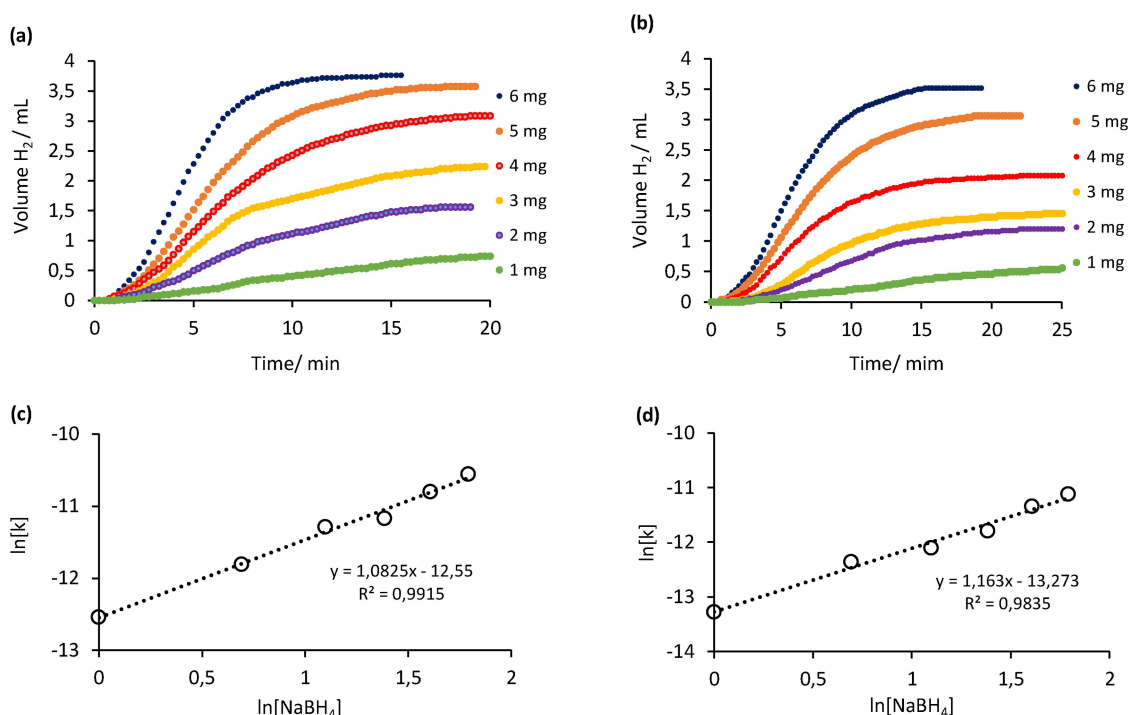
Figure 8. (a) and (b) Plots of volume of hydrogen vs time for the hydrolytic dehydrogenation of NaBH_4 catalyzed by 3a (0.0725 g, 0.026 mmol) and 3b (0.0340 g, 0.026 mmol), respectively; reactions were conducted in 200 mL water and the initial concentration of sodium borohydride varied ( [NaBH_4]_0 = 0.13, 0.26, 0.39, 0.52, 0.65, 0.78 mM); (c) and (d) plots of hydrogen generation rate versus concentration of sodium borohydride in logarithmic scale for (c) 3a and (d) 3b , respectively. Volumes measured are an average of three runs.
