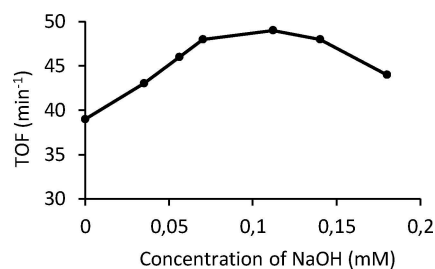
Figure 5. TOFs for the catalytic hydrolysis of 2 mL of an aqueous solution of NaBH 4 (0.021 g, 0.57 mmol) at 21 °C with 0.32 mol% 3a as a function of the sodium hydroxide concentration.
