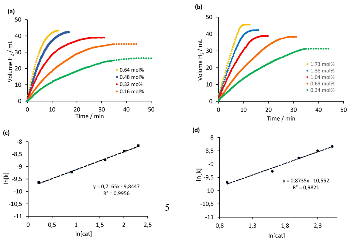
Figure 7. (a) and (b) Plots of volume of hydrogen vs time for the hydrolysis of 2 mL of 0.27 M \text{NaBH}_4 at 35^\circ\text{C} catalyzed by various concentrations of 3a and 3b , respectively; (c) and (d) plots of hydrogen generation rate vs concentration of catalyst in logarithmic scale for 3a and 3b , respectively. Volumes measured are an average of three runs.
