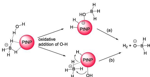
Figure 9. Proposed pathways for PtNP-catalyzed hydrolytic hydrogen evolution from NaBH_4 – via oxidative addition of an O–H in water involving the hydrogen-bonded surface-coordinated ensemble [H_3B-H-H-OH] followed by either (a) reductive elimination or (b) a \sigma -bond metathesis-type process.
