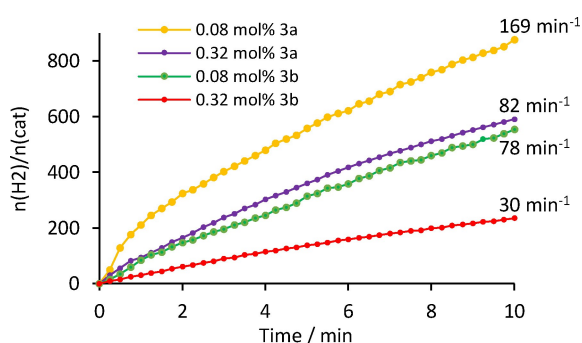
Figure 4. Hydrolytic release of hydrogen from NaBH 4 as a function of time at 30 °C catalyzed by 0.32 mol% and 0.08 mol% of 3a and 3b , respectively, and the corresponding initial TOFs.
