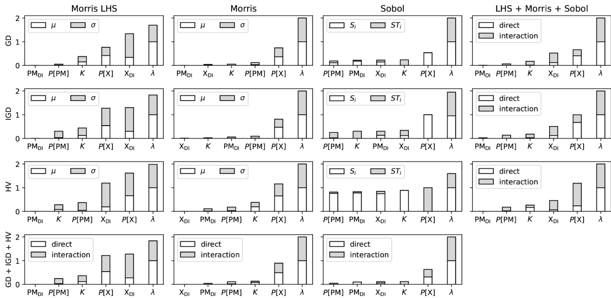
Fig. 7. NSGA-III algorithm's hyperparameters performance across all problems (functions). Rows 1, 2, and 3 respectively, show performance evaluated using GD, IGD, and HV metrics. Columns 1, 2, and 3, respectively indicate Morris LHS, Morris, and Sobol methods. The white color portion of a bar is direct influence normalized value in [0, 1] and gray color portion is interaction (total) influence value in [0, 1] . A larger height bar implies a higher influence, and hyperparameters in each subplot are arranged from low to high influence.
