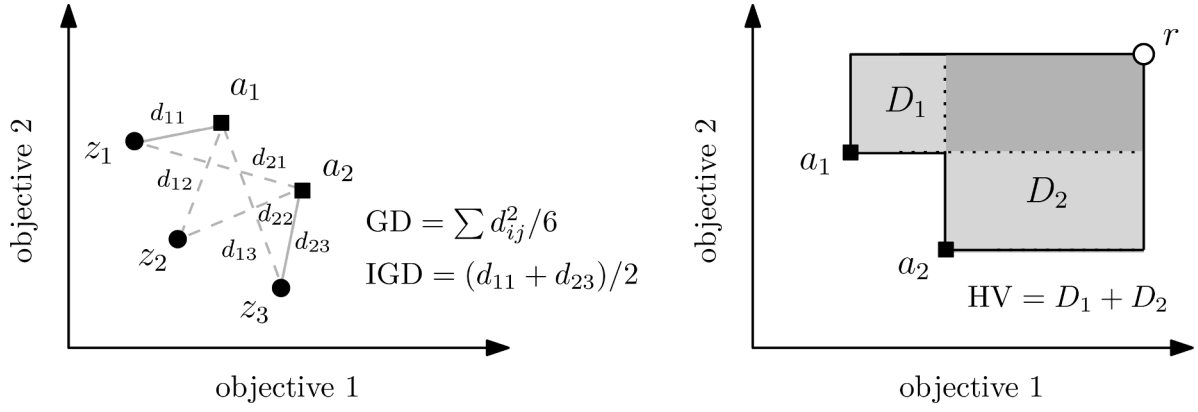
Fig. 1. Example of a 2D objective space and computation of GD, IGD, and HV metrics. The current Pareto front is \mathbf{A} = \{a_1, a_2\} and true Pareto front is \mathbf{Z} = \{z_1, z_2, z_3\} , and optimum of two-objective is a reference point r . The distance between two points is d_{ij} , and the area framed by a point with the reference point, r , is the area D_i .
