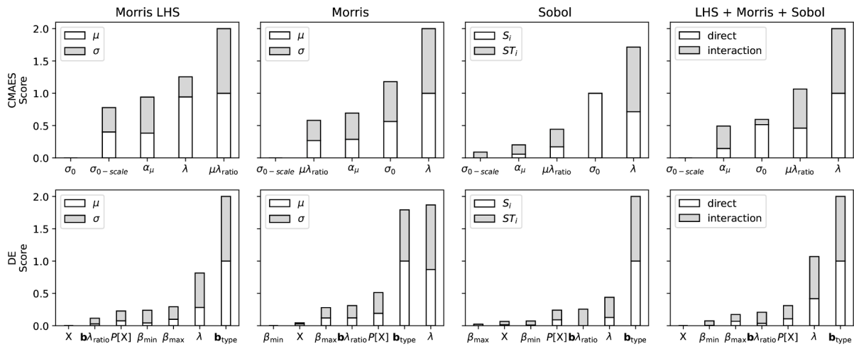
Fig. 4. Ordering (small to larger) of the sum of sensitivity analysis indices of single objective algorithms. CMA-ES (row 1) and DE (row 2) algorithms hyperparameters performance across all problems (functions). Columns 1, 2, and 3 respectively show performance evaluated using Morris LHS, Morris, and Sobol methods. The white color portion of a bar is the direct influence normalized value in [0, 1] and gray color portion is interaction (total) influence value in [0, 1] . Larger height bar implies a higher influence. Table 2 contains the hyperparameter name, definition and domain information.
