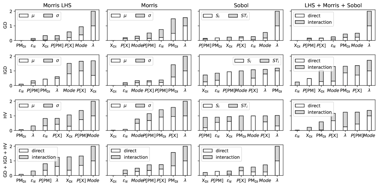
Fig. 10. MOEA/D algorithm’s hyperparameters performance across all problems (functions). Rows 1, 2, and 3, respectively, show performance evaluated using GD, IGD, and HV metrics. Columns 1, 2, and 3 respectively indicate metric Morris LHS, Morris, and Sobol methods. The white color portion of a bar is direct influence normalized value in [0, 1] and gray color portion is interaction (total) influence value in [0, 1]. A larger height bar implies a higher influence, and hyperparameters in each subplot are arranged from low to high influence.
