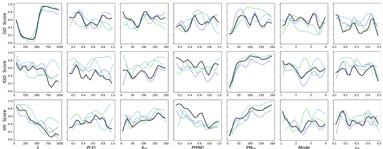
Fig. 11. MOEA/D algorithm average performance on 30 runs of each set of hyperparameters. MOEA/D hyperparameter (x-axis) against the mean metric value (y-axis). Rows 1, 2, and 3, respectively, are GD, IGD, and HV metrics. The scores are normalized between 0 and 1, where 0 is the best score for GD and IGD, and 1 is the best score for HV. A total of 590 samples were evaluated for the MOEA/D algorithm jointly by Morris LHS (blue lines), Morris (cyan lines), Sobol (green lines) methods. The hyperparameter values are arranged in 20 bins (lower values to higher values) across the x-axis. Each line in each plot connects the mean values of 20 bins of such samples. (For interpretation of the references to color in this figure legend, the reader is referred to the web version of this article.)
