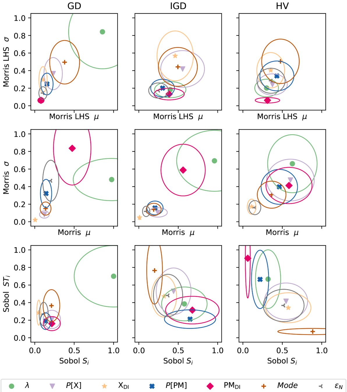
Fig. 9. MOEA/D hyperparameters sensitivity analysis. Columns 1, 2, and 3 respectively indicate performance metrics GD, IGD, and HV. Rows 1, 2, and 3, respectively, indicate Morris LHS, Morris, and Sobol methods. Legends of hyperparameter are shown at the bottom. Each hyperparameter is represented by a symbol and a color. An eclipse centered at a hyperparameter is the standard deviation of its influence and direction of its influence. Further apart a hyperparameter in the diagonal direction from the origin (0,0), the higher its importance to the algorithm. A larger width of the eclipse in the x-axis direction means more variation in the direct influence of a hyperparameter, and a larger height in the y-axis direction means variation in total (or interaction) influence. Supporting statistical tests and clustering analysis are provided in supplementary Sections A and B.
