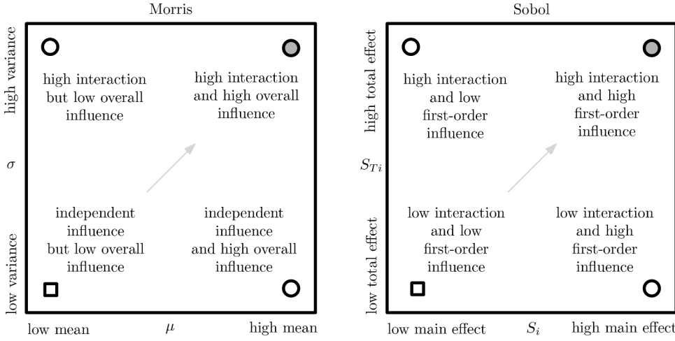
Fig. 2. Morris (left) and Sobol (right) indices interpretation. Top right corner circle in dark gray is the ideal case where a hyperparameter has high individual influence and high interaction (or total effect). Circles in white at the top left and bottom right corners are cases that have high importance in at least one direction. Bottom left square in white shows the least ideal case where hyperparameters are non-influential, and fixing them at any values within their defined domain will not influence the algorithm's performance. Arrow along the diagonal direction indicates the order of the hyperparameters' importance and influence.
