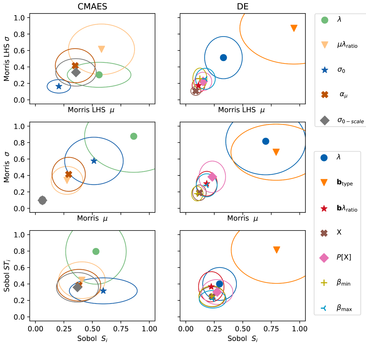
Fig. 3. Single objective algorithms sensitivity analysis. CMA-ES and DE hyperparameters sensitivity analysis are shown in column 1 and column 2, respectively. Rows 1, 2, and 3, respectively, indicate Morris LHS, Morris, and Sobol methods. The upper right legend belongs to CMA-ES and the lower right to DE. A symbol and a color represent each hyperparameter. An eclipse centered at a hyperparameter is the span of the standard deviation of the influence along with direct and interaction influences. A larger width of the eclipse of a hyperparameter in the x-axis direction means more variation in direct dominance of that hyperparameter, and a larger height in the y-axis direction means its variation in total (or interaction) influence. In each plot, the further apart a hyperparameter in the diagonal direction from the origin (0,0) is, the higher its importance to the algorithm. CMA-ES hyperparameter \lambda , \mu\lambda_{ratio} , \sigma_0 , \alpha_\mu , and \sigma_{0-scale} respectively are population size, percentage of the population for covariance matrix, initial step size, learning rate, and convergence speed controller. DE hyperparameters \lambda , \mathbf{b}_{type} , \mathbf{b}\lambda_{ratio} , X , P[X] , \beta_{min} , and \beta_{max} respectively are population size, base vector selection type (mutation type), percentage of the population for base vector selection, crossover-type, crossover probability, minimum acceleration coefficient, and maximum acceleration coefficient. Table 2 contains the hyperparameter name, definition and domain information. Supporting statistical tests [79] between direct and interaction effects and clustering analysis are provided in supplementary Sections A and B.
