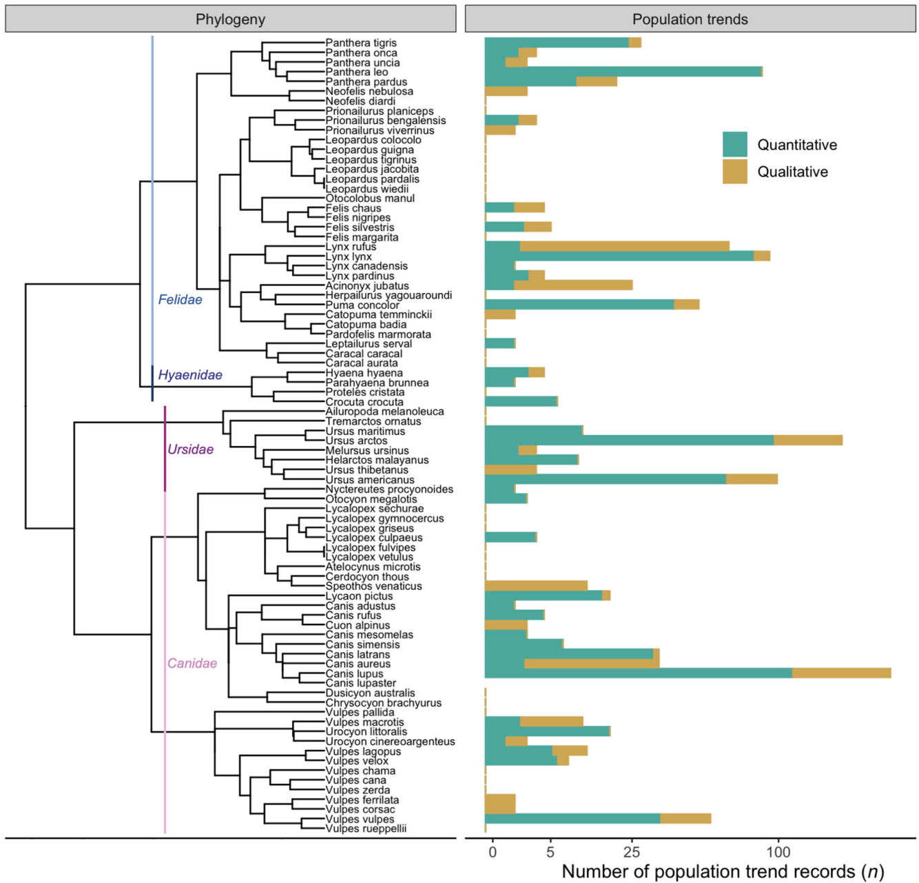
FIGURE 1 Number of population trend records per studied species, shown across the Carnivora phylogeny. The tree represents four taxonomic families: Canidae, Ursidae, Felidae and Hyaeonidae. We show records for both quantitative (teal) and qualitative (gold) trends. We use a subset of the Upham et al. (2019) mammal phylogeny, restricted to relevant clades and with small amendments to accommodate differences between the phylogeny and International Union for Conservation of Nature (IUCN) taxonomy – see Supporting Information: Using the IUCN taxonomy with a phylogeny
