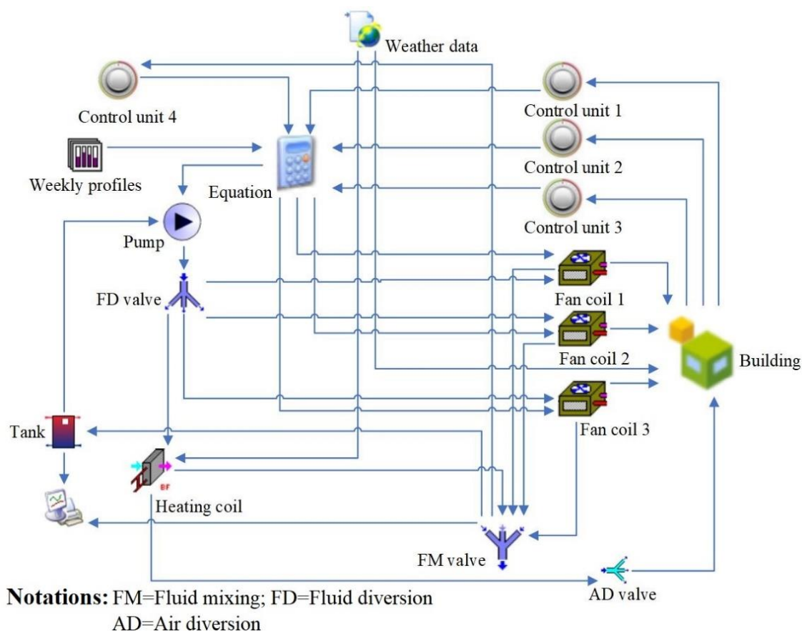
Figure 5. Components and links of space heating distribution system in TRNSYS.
