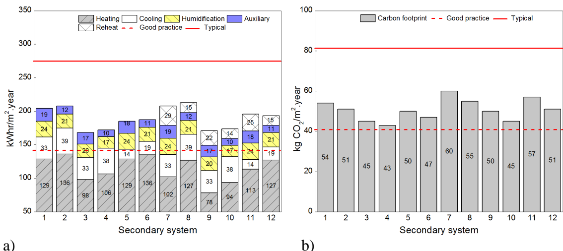
a) b) Figure 6: Third primary systems-CCHP (absorption chiller with CHP) a: energy consumption b: energy related CO 2 emissions.
