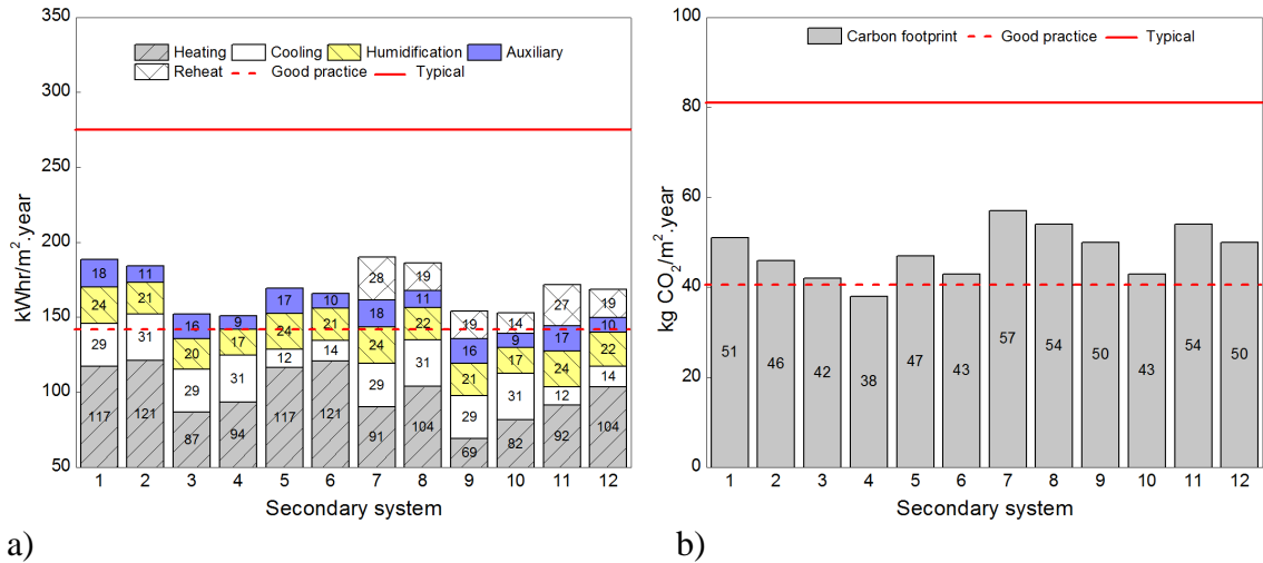
a) b) Figure 5: Second primary systems (gas boiler with absorption chiller) a: energy consumption b: energy related CO 2 emissions.
