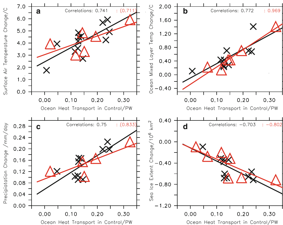
Fig. 6 Relationships between changes ( 2 \times \text{CO}_2 - \text{Control} ) in Arctic variables and the time mean Ocean Heat Transport at 70N ( black : Global ( T otal N O cean H eat T rans), red : Atlantic [ A tl O cean H eat T rans])—across all available models. a Air
