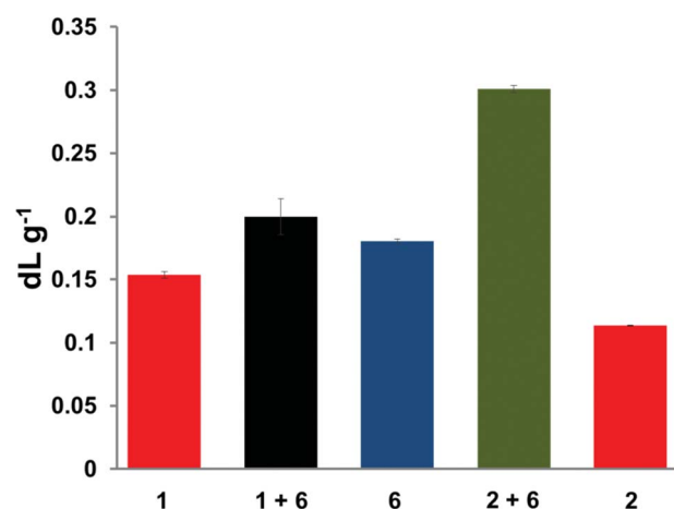
Fig. 3 Inherent viscosities of individual polymers ( 1 , 2 and 6 ) and the equimolar (with respect to binding motifs) polymer blends ([1 + 6] and [2 + 6]) at 10 mg mL -1 in chloroform-hexafluoroisopropanol (9 : 1, v/v). Viscosities are the mean of four repeat measurements in each case.
