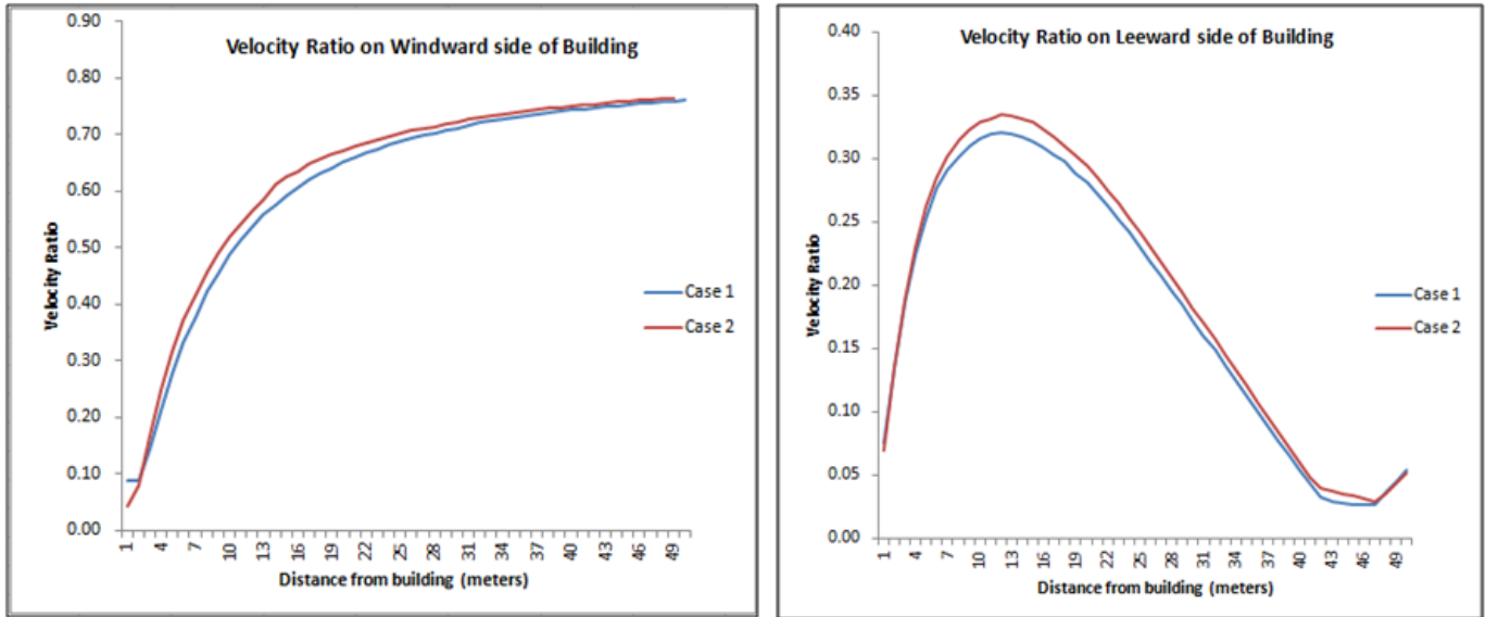
Figure 7: Velocity ratios along the central line on windward and leeward sides of the building
