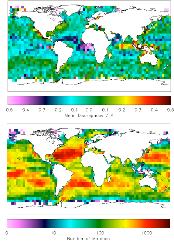
Figure 4. Upper panel: Mean discrepancy map for a single-view split-window SST estimator, adjusted for the SST skin effect and near-surface stratification, relative to drifting buoy SST. This is an estimate of the geographical variation in bias in the SST estimates. The SSTs are for the “nadir two-channel” retrieval for all matches found for a series of three Along Track Scanning Radiometers (ATSRs) between 1991 and 2011. (Note that the ATSRs are dual-view sensors; the geographical variations seen here in the tropics are greatly reduced when taking advantage of dual-view capability.) Lower panel: number of ATSR/drifting-buoy matches obtained over two decades. The marked variation in density of matches arises from the combination of drifting buoy deployment patterns and prevalence of cloud cover. Matches are particularly few in the highest latitudes and the tropical warm pool (round Indonesia), where both these factors are unfavourable.
