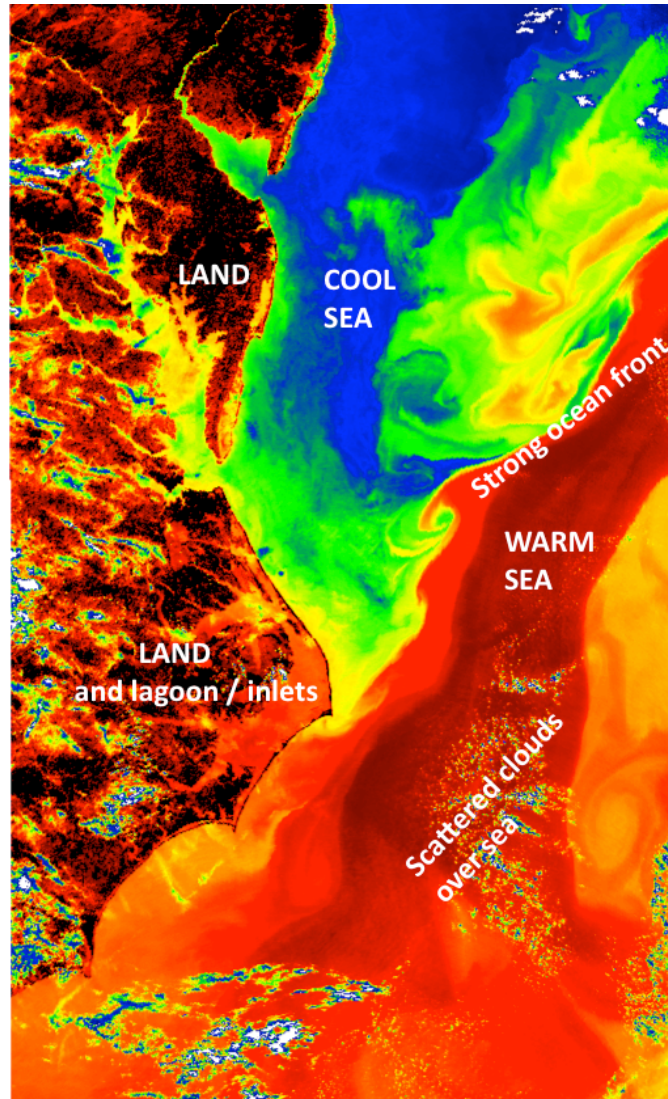
Figure 1. Image at thermal window wavelength of 11 \mu\text{m} of US Eastern seaboard including Cape Hatteras and Pimlico Sound, obtained by the second Along Track Scanning Radiometer. The width of the image is about 512 km and the pixel resolution is 1 km. Ocean features are reasonably well resolved, with smooth contiguous variations in surface temperature reflected in the image brightness temperature, except where there are scattered, cooler clouds that are often not fully resolved. Land is also more heterogeneous, and, this being a day time image, warmer than the sea in many areas. Image obtained from URL1 and adapted by the author.
