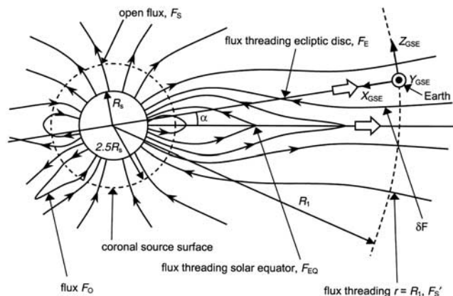
Figure 1. Idealized schematic of open solar flux near solar minimum. The total flux threading of the coronal source surface (dot-dashed line, at r \approx 2.5R_s ) is F_s and contains the flux F'_s = (2\pi R_1)|B_{rE}| that threads a heliocentric sphere of radius R_1 = 1 AU, plus the flux F_{EQ} that threads the solar equator inside the Earth's orbit and the open flux F_O that cuts neither the 1 AU sphere nor the ecliptic plane. The flux F_E threading the ecliptic plane at r < R_1 differs from F_{EQ} by the flux \delta F . Field lines contributing to the fluxes F_s , F'_s , F_{EQ} , F_O , F_E , and \delta F are all labelled.
