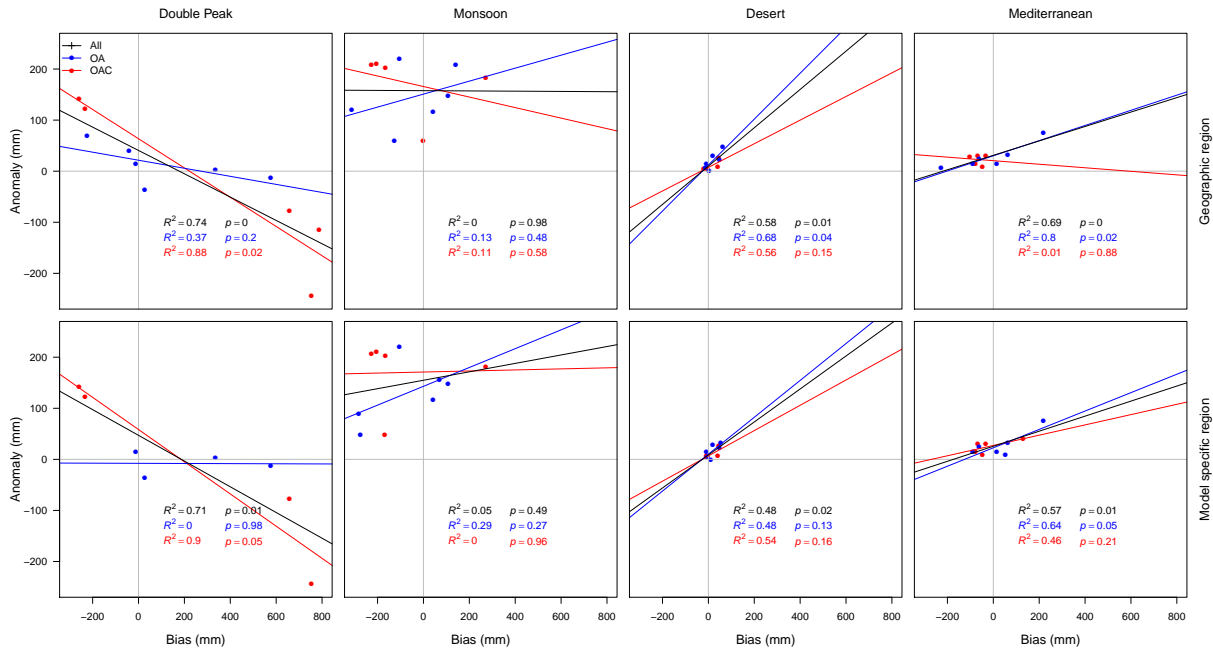
Fig. 7. Relationship between biases in the piControl simulation of mean annual precipitation (mm) and mid-Holocene precipitation anomalies ( midHolocene – piControl ) as simulated by each of the CMIP5 models for each of the precipitation regimes (Double Peak, Monsoon, Desert, Mediterranean). The upper panels show biases and anomalies calculated for specific latitudinal bands from the modern observed spatial extent of each regime (geographic region). The lower panels show biases and anomalies calculated for the region identified as characterized by a given regime in each model and simulation (model specific region). The regressions are calculated for all models (All: black), for the coupled ocean–atmosphere models (OA: blue) and for the carbon-cycle models (OAC: red).
