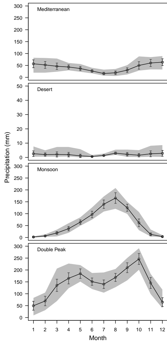
Fig. 1. Observed seasonal cycle of precipitation in each of the defined climate zones, using the CRU T3.1 data set (Harris et al., 2014). The mean precipitation each month (mm) is shown by the black line, with the standard deviation shown by the bars. The grey shading shows the maximum and minimum rainfall experienced within the observation period (1961–1990). Note that the scale for the desert region differs from that used for the other regions. Months are numbered consecutively from January (1) through to December (12).
