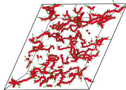
(c) \lambda = 6.17 , Newtonian regime
