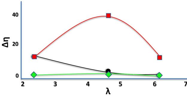
FIG. 10. A schematic of MVE in Newtonian regime for different dipolar interaction strengths. The MVE when the field is oriented in (1) the flow direction is shown as circles (2) the gradient direction of flow is shown as squares (3) vorticity direction is denoted by diamonds.
