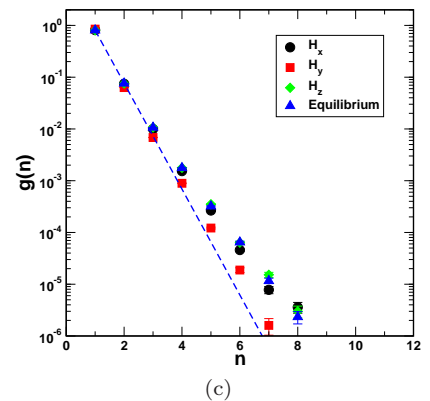
FIG. 11. For \lambda \approx 2.37 with applied field H in shear thinning regime: (a) The configurational viscosity \eta_{\text{conf}} , the rotational viscosity \eta_{\text{rot}} and the total viscosity \eta_{\text{tot}} = \eta_{\text{conf}} + \eta_{\text{rot}} as a function of strength of the magnetic field H are shown as circles, squares and diamond symbols, respectively. Top panel: Viscosities when the field is oriented in the flow direction, middle panel: when the field is oriented in the gradient of the flow direction, bottom panel: when the field is oriented in the vorticity direction. (b) The connectivity C(n_c) as a function of n_c for different orientations of magnetic field (c) Cluster size distribution g(n) as a function of n at different orientations of magnetic field. Exponential fit to the data is given as dashed line. All structural analysis are performed with a fixed magnetic field strength of H = 2.0 . Explanation is given in Sec. V B 1.
