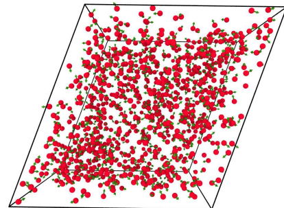
(b) \lambda = 2.37 , Shear thinning regime
