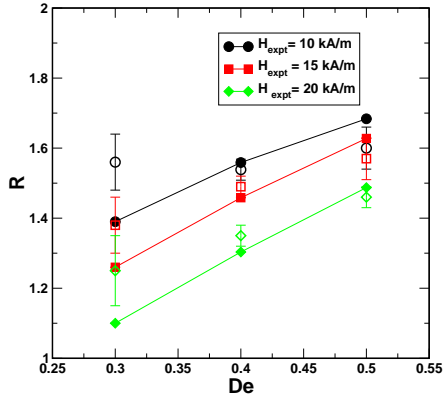
FIG. 19. The ratio R of \Delta\eta_{\parallel} and \Delta\eta_{\perp} as a function of dimensionless shear rate for different magnetic field strengths (solid and open symbols correspond to simulation and experiment, respectively).
