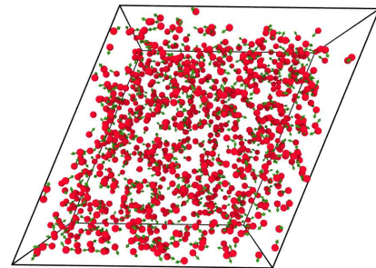
(a) \lambda = 2.37 , Newtonian regime
