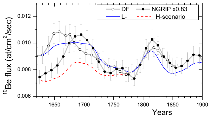
Fig. 15. Depositional flux of ^{10}\text{Be} in polar ice. All data are pseudo-decadal and 25-yr low-pass smoothed because of strong high-frequency noise. Grey curves depict the fluxes measured at Dome Fuji (DF) in Antarctica (Horiuchi et al. 2007), and at NGRIP (scaled as 0.83), Greenland (Berggren et al. 2009). Error bars are estimates of both statistical and systematic errors. The blue and red curves depict the modelled ^{10}\text{Be} depositional fluxes for the L- and H-scenarios (see text for details), respectively.
