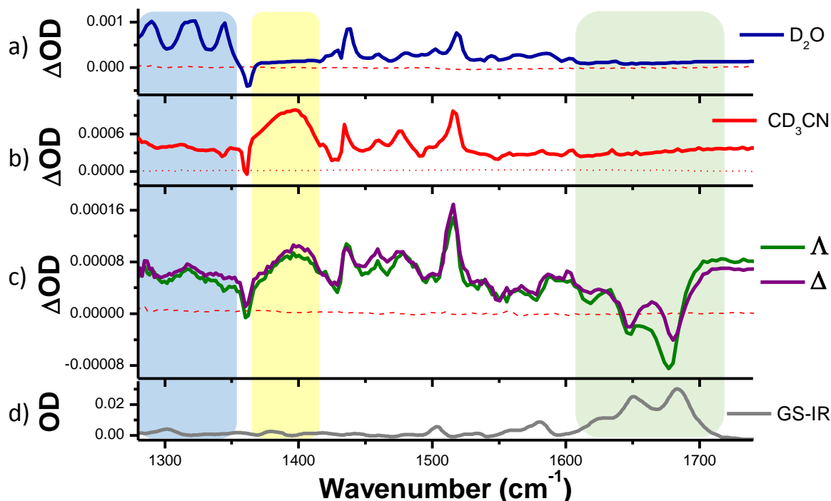
Fig. 8 TRIR spectra recorded 35 ps after 400 nm excitation of a) 1 \cdot 2\text{Cl} (500 \mu\text{M} ) in \text{D}_2\text{O} , b) 1 \cdot 2\text{PF}_6 (500 \mu\text{M} ) in \text{CD}_3\text{CN} and c) \Delta - and \Lambda -[1]2CF (400 \mu\text{M} ) and a duplex DNA oligonucleotide d(\text{TCGGCGCCGA})_2 (500 \mu\text{M} duplex) and d) FTIR spectrum oligonucleotide d(\text{TCGGCGCCGA})_2 (500 \mu\text{M} duplex) in deuterated potassium phosphate buffer (50 mM) pH 7. The blue and yellow coloured regions highlight the characteristic transient bands for the excited state of 1 , while the green coloured region highlights the bands associated with the base DNA base pairs.
