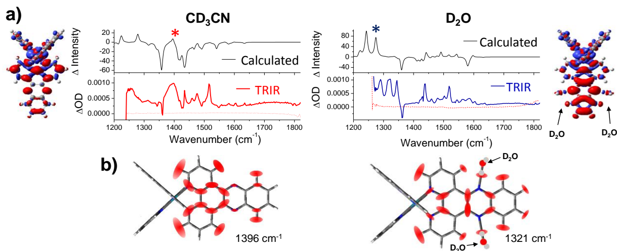
Fig. 7 a) Simulated difference spectra compared with the experimental TRIR spectra of 1 in acetonitrile (left column); and 1 -(D 2 O) in water (right column). In the experimental spectra, wavenumbers below 1250 cm -1 were inaccessible due to strong absorbance of both solvents in this region. Structural inserts show electron density difference map (iso level 0.0008) between the lowest energy triplet state of 1 minus the electron density of the equivalent singlet ground-state at the same geometry in acetonitrile (left hand side) and for 1 -(D 2 O) in water (right hand side). (The red and blue volumes indicate the regions where the electron density is respectively higher and lower in the triplet state compared to the ground state); b) Graphical illustration of the in-plane vibrational modes of the marker bands of the “bright” and “dark” states of 1 at 1396 cm -1 in CD 3 CN and 1321 cm -1 in D 2 O (marked with asterisks in the spectra). Red ellipsoids indicate the regions of largest atomic displacement. Animations of these vibrations can be found online in the ESI † (Animation 1-CD 3 CN and Animation 2-D 2 O).
