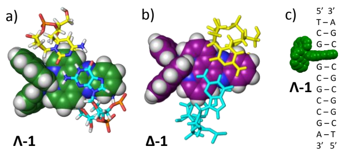
Fig. 9 a) Angled intercalation by \Lambda - 1 into the terminal CC/GG step in d(\text{CCGGATCCGG}) . 71 Note that the dppz is located under the purine (guanine) bases. Bases are coloured according to atom type with nitrogen in blue, oxygen in red, hydrogen in white and phosphorus in orange. Carbon atoms are cyan for guanine, yellow for cytosine and green for \Lambda - 1 ; b) a hypothetical model of an angled CC/GG intercalation site for \Delta - 1 , constructed by direct manipulation of the crystal structure, to illustrate the difference in binding if the dppz group were directed further towards the pyrimidine bases (cyan). Purine bases are drawn in cyan; c) schematic diagram of the binding of \Lambda - 1 at the \text{G}_3\text{G}_4/\text{C}_7\text{C}_8 step.
