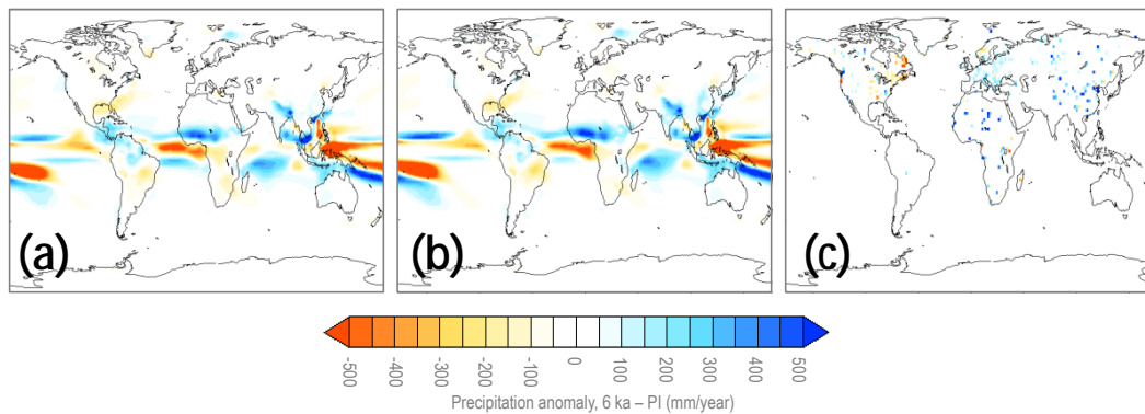
Figure 15. Mid-Holocene minus pre-industrial precipitation anomalies: (a) annual mean precipitation anomalies from the control experiment; (b) annual precipitation anomalies from the KK10 experiment; (c) Bartlein et al. (2011) pollen-based reconstructions of the mean annual precipitation anomaly.
