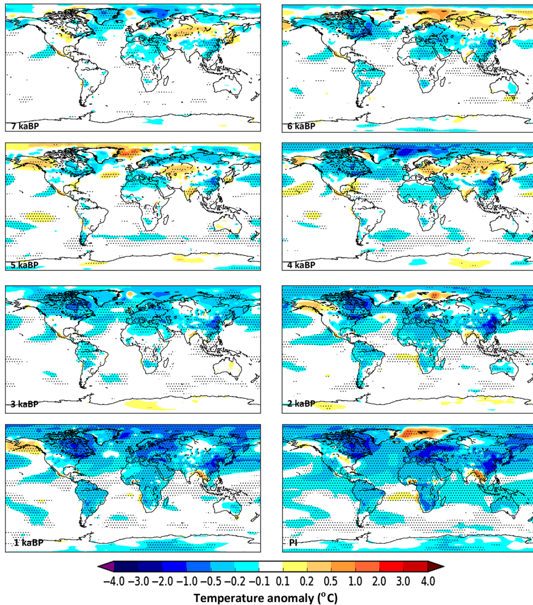
Figure 3. DJF temperature anomalies ( ^{\circ}\text{C} ) for KK10 minus control at time slices from the late pre-industrial period (1850 CE) to 7 ka BP. The stippling indicates grid boxes where the anomalies are significant at the 95 % level using Wilcoxon rank sum statistical analysis.
