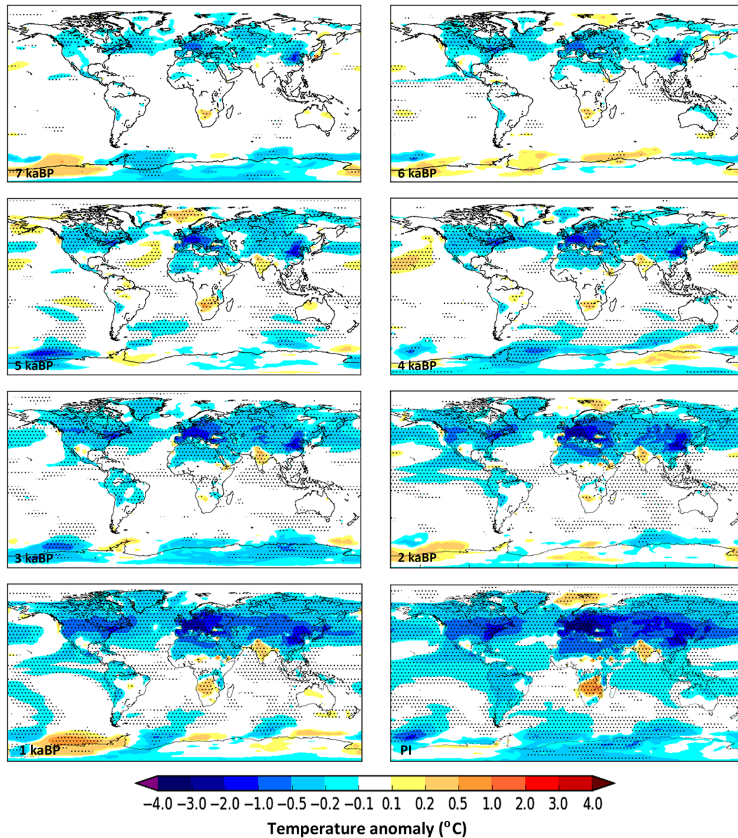
Figure 2. JJA temperature anomalies (°C) for KK10 minus control at time slices from the late pre-industrial period (1850 CE) to 7 kaBP. The stippling indicates grid boxes where the anomalies are significant at the 95 % level using Wilcoxon rank sum statistical analysis.
