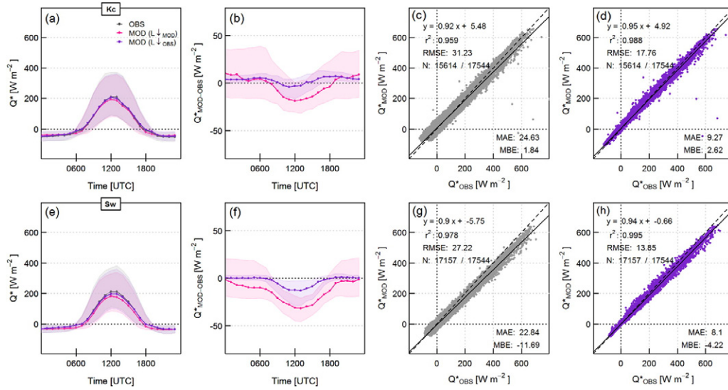
Fig. 6. (a, e) Median diurnal cycle and inter-quartile range for modelled and observed net all-wave radiation Q^* ; (b, f) difference between modelled and observed Q^* by time of day; (c, g) scatter plot of modelled versus observed Q^* . Results are also shown (in purple) for the case where observed L_i is provided with the meteorological forcing data (d, h) rather than modelled.
