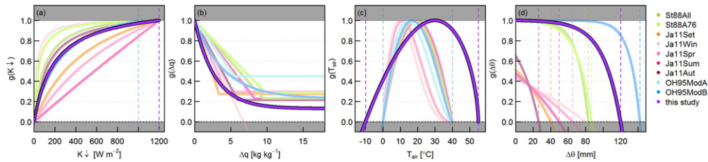
Fig. A1. Relations for the dependence of surface conductance on (a) incoming shortwave radiation K_{\downarrow} , (b) specific humidity deficit \Delta q , (c) air temperature T_{air} and (d) soil moisture deficit \Delta\theta for this study and from literature (St88 - Stewart (1988): all data (All) and 1976 data only (A76); OH95 - Oginck-Hendriks (1995): linear dependence on \Delta q (ModA) and exponential dependence on \Delta q (ModB); Ja11 - Järvi et al. (2011): recommended values based on the whole data set (Set) and for each season separately (Win, Spr, Sum, Aut)).
