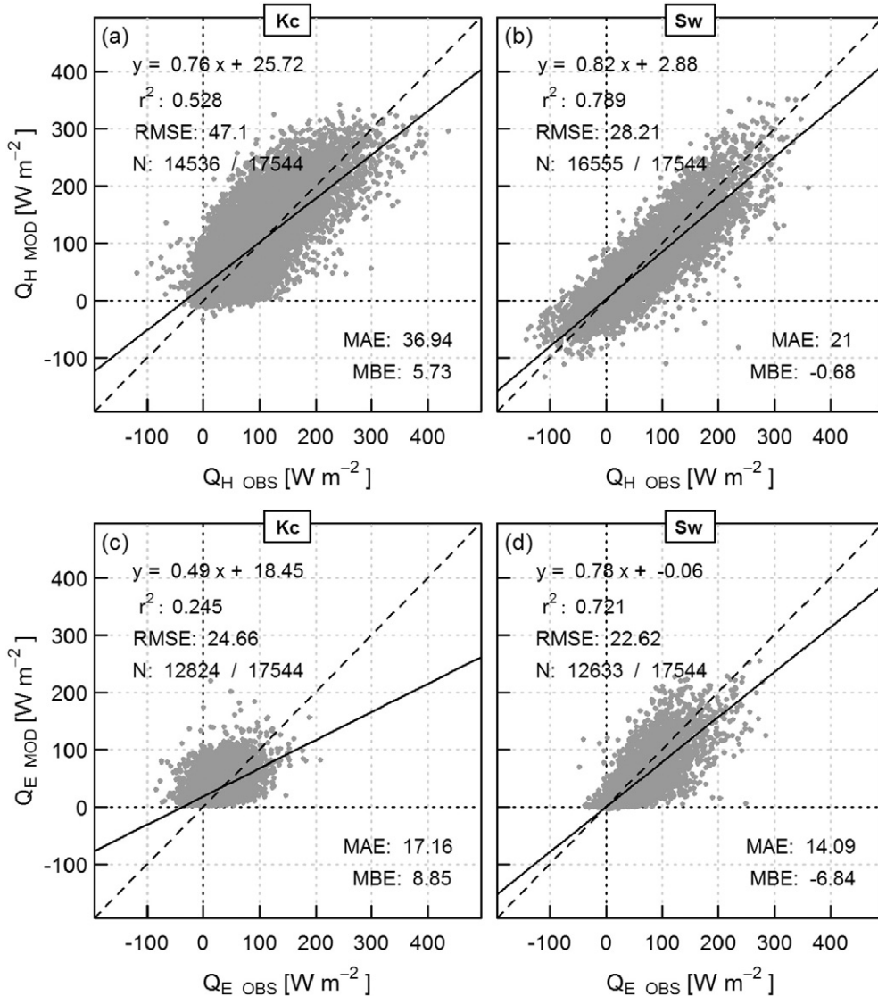
Fig. 12. Modelled versus observed (a, b) sensible heat flux Q_H and (c, d) latent heat flux Q_E for London (Kc) and Swindon (Sw).
