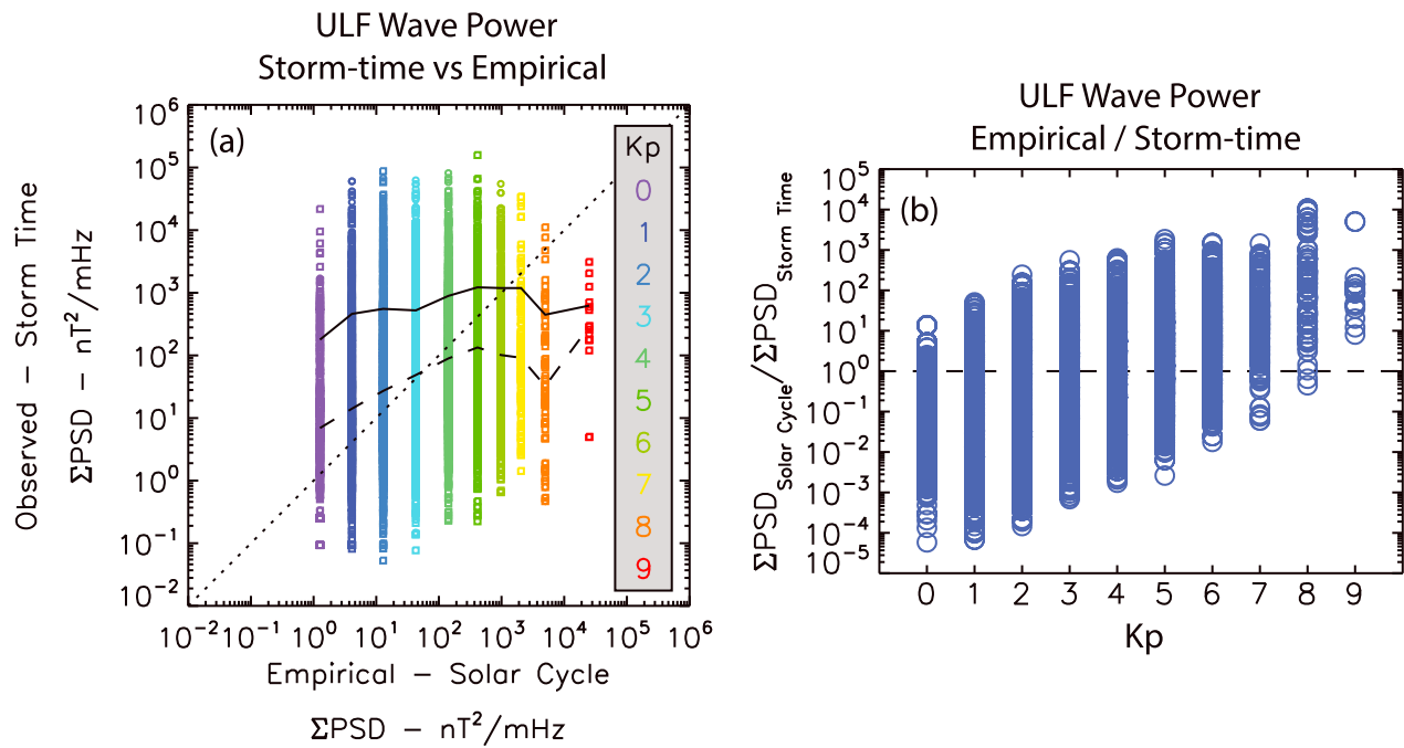
Figure 1. A comparison between the observed storm-time and solar cycle averaged \Sigma\text{PSD} as a function of Kp . (a) Observed storm-time versus empirical solar cycle average \Sigma\text{PSD} , overlotted are the median (dashed) and mean (solid) storm-time ULF PSDs, \Sigma\text{PSD} , as a function of Kp . (b) The ratio of solar cycle \Sigma\text{PSD} to storm-time \Sigma\text{PSD} as a function of Kp .
