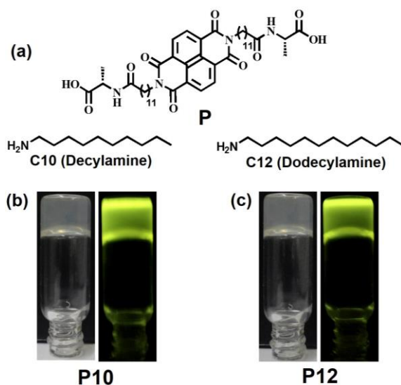
Figure 1. (a) Chemical structures of the peptide ( P ) and amines decylamine (C10) and dodecylamine (C12). (b) and (c) Photographs of two-component hydrogels P10 ( P with C10) and P12 ( P with C12) at a 1:2 molar ratio of peptide: amine in daylight (left side) and under UV lamp (right side) (365 nm) respectively.
