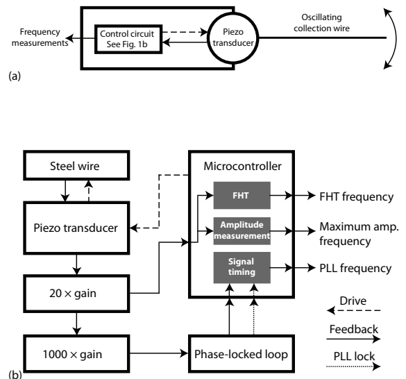
FIG. 1. (a) Sketch of the oscillating microbalance collector. (b) Block diagram to illustrate the main components and signal flow. Dashed lines show optional drive provided to the piezo transducer, dotted lines show the PLL 'lock' state signal, and solid lines show the signal received from the wire vibration. White boxes indicate hardware and grey boxes indicate software. Signal flow and component definitions are described in the text.
