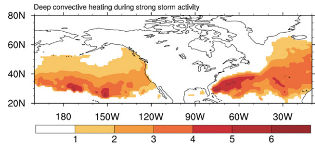
FIG. 6. Mean heating from deep convection during strong-storm activity averaged between 900 and 100 hPa in the Northern Hemisphere during DJF for 1980–2010. Contour interval is 1.0 \text{ K day}^{-1} . Regions outside the all-storm-track regions are masked out.
