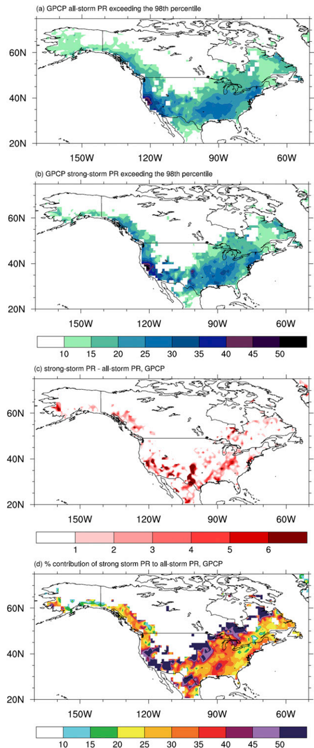
FIG. 13. As in Figs. 11b–e, but for GPCP precipitation for 1999–2010.
