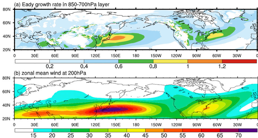
FIG. 3. (a) The 1980–2010 DJF Eady growth rate average for the 850–700-hPa layer. Values exceeding 0.2 \text{ day}^{-1} are shaded at 0.2 \text{ day}^{-1} intervals. Masked areas over the continents indicate regions where the land extends above the 850-hPa surface. (b) Zonal mean wind at 200 hPa. Values exceeding 15 \text{ m s}^{-1} are shaded.
