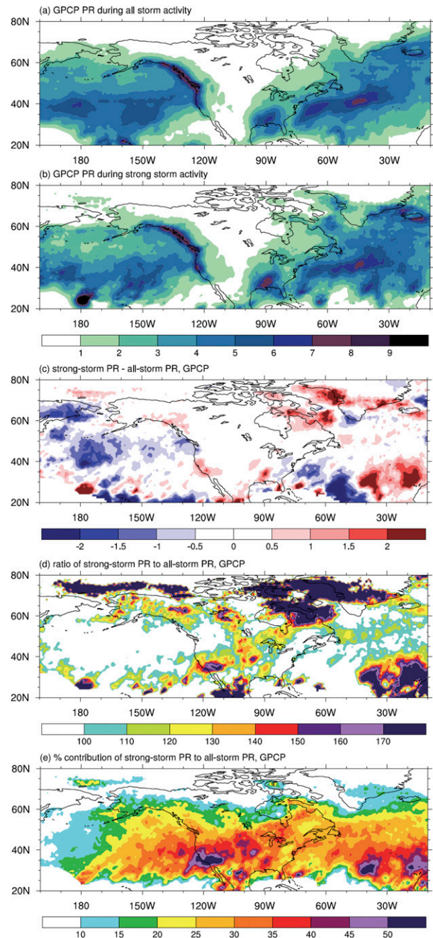
FIG. 12. As in Fig. 10, but for GPCP precipitation for 1999–2010.
