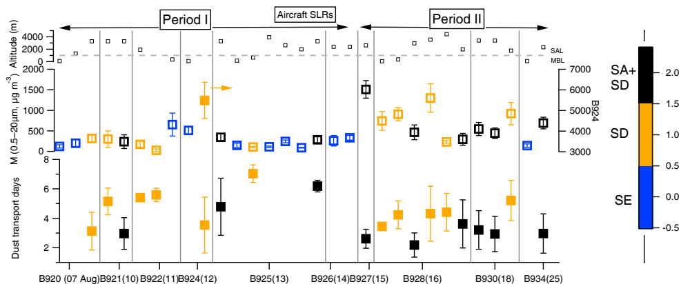
Figure 9. A summary of altitude, potential dust age and aerosol mass ( 0.5\text{--}20\mu\text{m} ) for all aircraft SLRs. Note the aerosol mass for flight B924 is shown on the right axis. The numbers in brackets show the dates of flights in August. The grey dashed line indicates the layer height separating the SAL and MBL.
