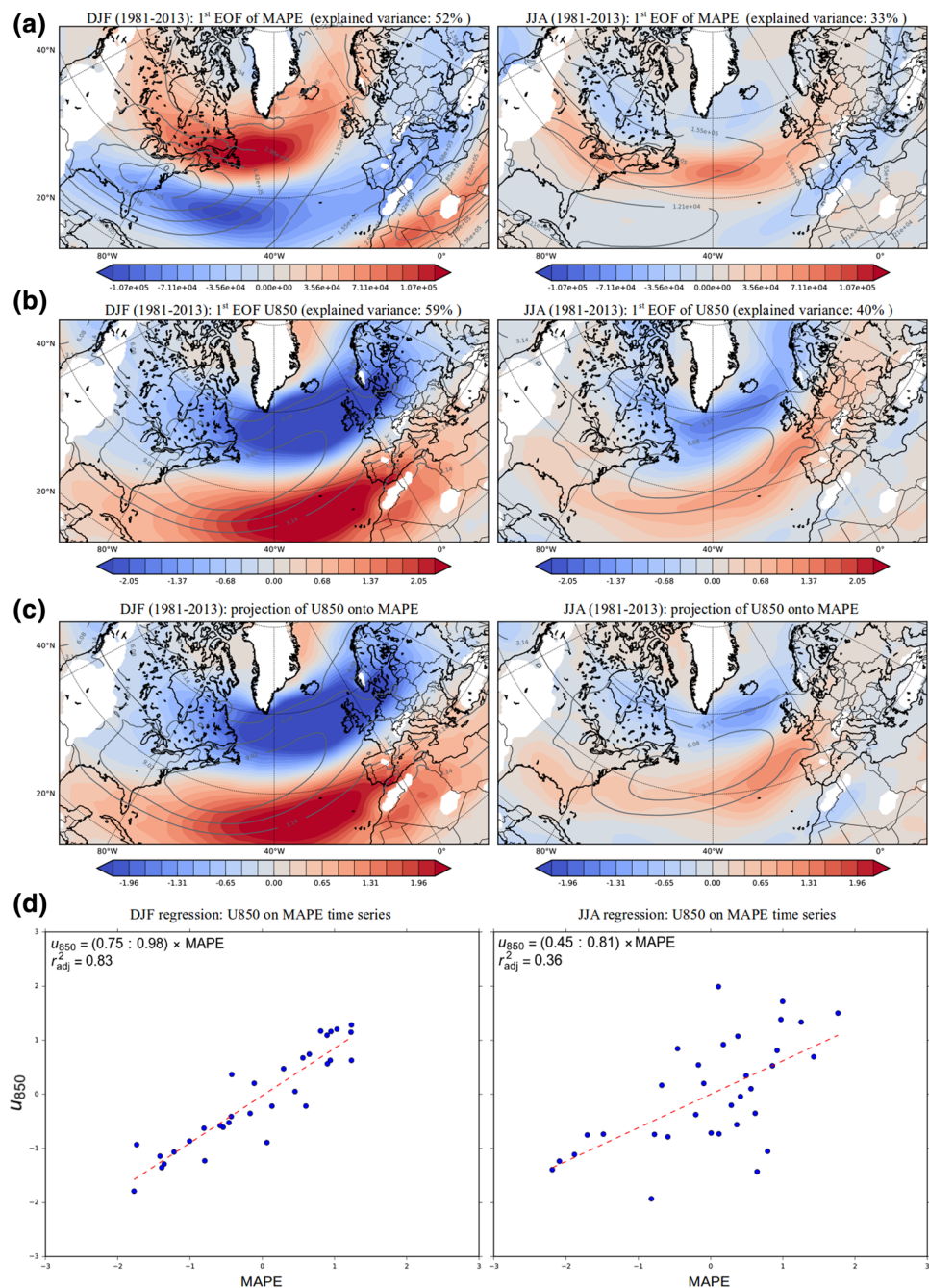
Fig. 4 The filled, colored contours show a the 1st EOF of seasonal-mean vertically-averaged baroclinic mean available potential energy (800–200 hPa); b the 1st EOF of 850 hPa seasonal-mean zonal wind; c the projection of 850 hPa seasonal-mean zonal wind anomalies onto the time series associated with the 1st EOF of the vertically-averaged seasonal-mean baroclinic mean available potential energy. The gray, unfilled contours in a show the climatology of the vertically-averaged seasonal-mean MAPE, while the ones in b, c show the climatology of 850 hPa seasonal-mean zonal wind. The units of MAPE are \text{J}/\text{m}^2 and zonal winds are \text{m}/\text{s} . d Least squares regression of the 850 hPa seasonal-mean zonal wind's 1st EOF's time series onto vertically-averaged seasonal-mean MAPE's 1st EOF's time series. The time series have been standardized. Left: DJF. Right: JJA
