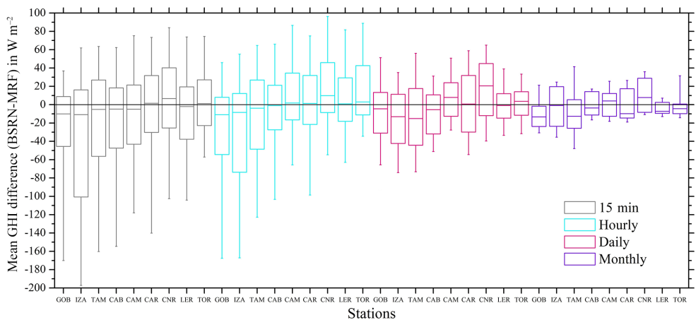
Figure 6. Mean GHI differences in \text{W m}^{-2} derived by MRF as compared to the BSRN stations for each time horizon. The boxes represent the 25th and 75th percentiles, while the in-box lines represent the median of the difference of each station. The upper and lower whiskers represent the minimum and maximum error values.
