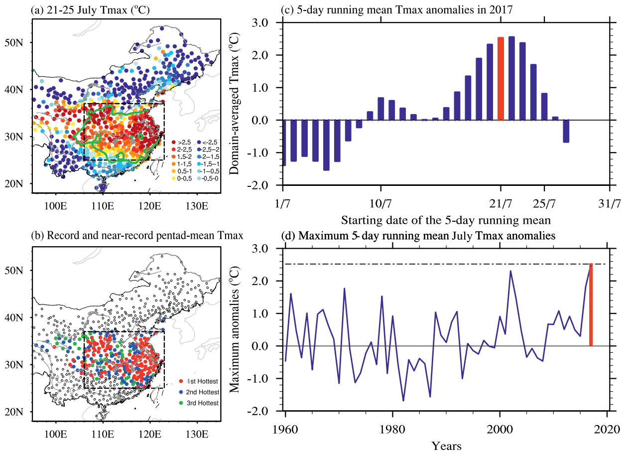
FIG. 1. (a) Observed pentad-mean (21–25 Jul 2017) Tmax anomalies (°C) relative to the 1961–90 climatology for the maximum 5-day mean Tmax. The green contour indicates the 35°C-isoline of mean Tmax during this pentad. Central eastern China is shown by the dashed rectangle. (b) Spatial distribution of stations that registered record- and near-record (since 1960) pentad-mean July Tmax during 21–25 Jul 2017. (c) Observed overlapping pentad-mean Tmax anomaly averaged over central eastern China during July 2017. Each value is indexed by the first day of the pentad. (d) Observed maximum 5-day mean Tmax anomaly averaged over central eastern China in each July over 1960–2017. The red vertical line labels the 2017 event, and the dashed line indicates its anomaly.
