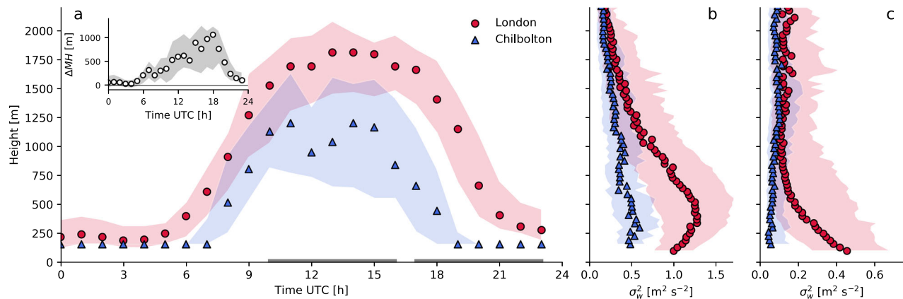
Fig. 5 Doppler lidar derived vertical velocity variance and mixing height. a Median mixing height (MH) and median hourly difference ( \Delta MH); ( b,c ) median vertical velocity variance between b 10:00 and 16:00 UTC and c 17:00 and 23:00 UTC for London at WCC (red) and Chilbolton (blue) with interquartile ranges (shaded). For available cumulus days between 1 May 2011 to 31 August 2011 ( n_{\text{days}} = 69 )
