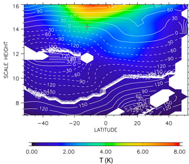
FIG. 27-5. Mean amplitude and phase structure of the diurnal, eastward-propagating tide of wavenumber 3 (DE3) in the range of altitude 7–16 scale heights ( \sim 49 – 112 km) obtained via coherence analysis of SABER data over the period 2002–17 (see Garcia et al. 2005). The base point for the coherence analysis is denoted by the red cross; results are shown only where the squared coherence statistic is significant at the 95% level. As can be seen from the phase structure, the DE3 tide is predominantly equatorially antisymmetric below 14 scale heights ( \sim 98 km), and symmetric above that level. This suggests that forcing of DE3 projects onto both antisymmetric inertia–gravity and symmetric Kelvin modes. The amplitude is large (8 K) in the lower thermosphere.
