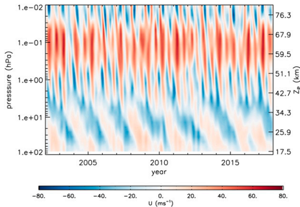
FIG. 27-7. Equatorial zonal-mean zonal wind over the period 2002–17 as estimated from SABER geopotential data (after Smith et al. 2017). The stratospheric QBO and mesospheric SAO dominate the variability of the wind. The interruption of the 2016 descending westerly phase of the QBO near 40 hPa in 2016 (Osprey et al. 2016) can be clearly seen.
