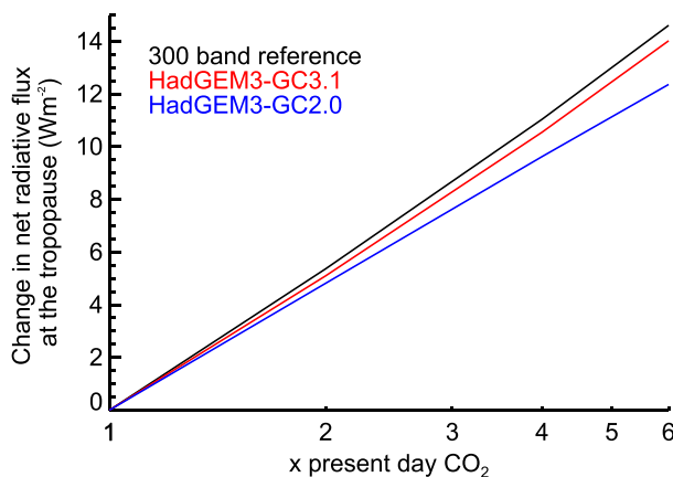
Figure 3. \text{CO}_2 radiative forcing at the tropopause from offline radiative transfer calculations using the treatment of greenhouse gas absorption in (blue) HadGEM3-GC2.0 and (red) HadGEM3-GC3.1 compared to a (black) reference 300 band case. Note that the x axis has a logarithmic scale. Each calculation is averaged over four different profiles with varying humidities following the method of Pincus et al. (2015).
