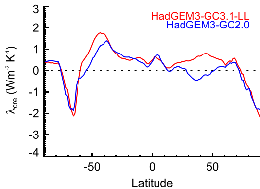
Figure 2. Zonal-mean cloud feedback parameter ( \lambda_{\text{CRE}} ) in the HadGEM3-GC3.1-LL and HadGEM3-GC2.0 abrupt-4xCO 2 simulations.
