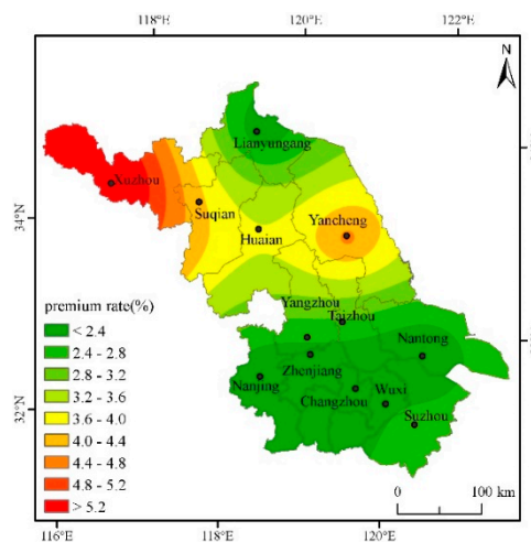
Figure 2. Distribution of actuarially fair premium rate for each city when the deductible amount is 2.5%.
