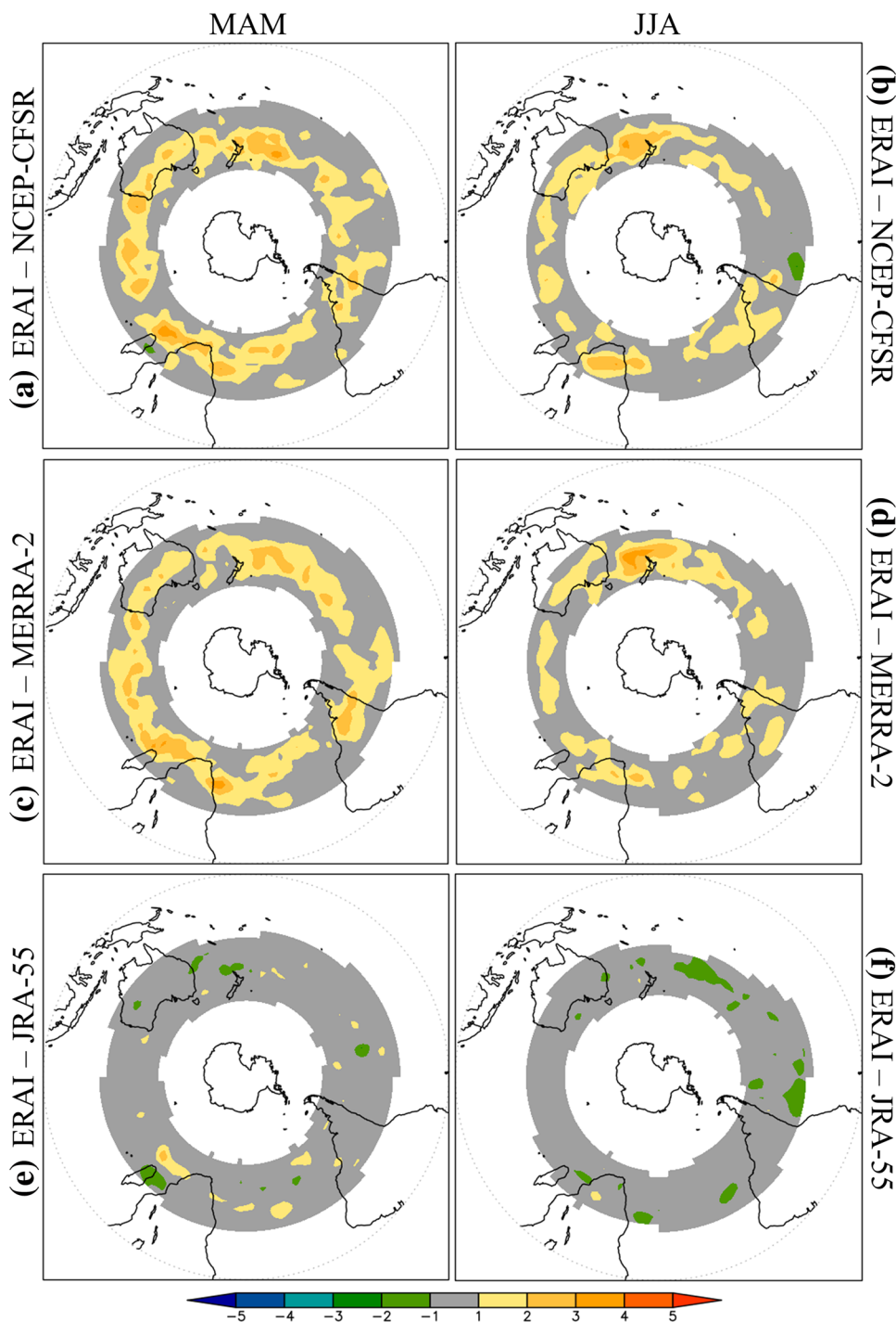
Fig. 2 Differences of track density for the \xi_{300} Cut-off lows in the Southern Hemisphere, between ERA-Interim and NCEP-CFSR (top), ERA-Interim and MERRA-2 (middle), and ERA-Interim and JRA-55 (bottom) for the austral autumn (left panel) and winter (right panel). The analysis is performed for the 30-year period (1980–2009). Units is number per unit area, the unit area is equivalent to a 5^\circ spherical cap ( \cong 10^6 \text{ km}^2 )
