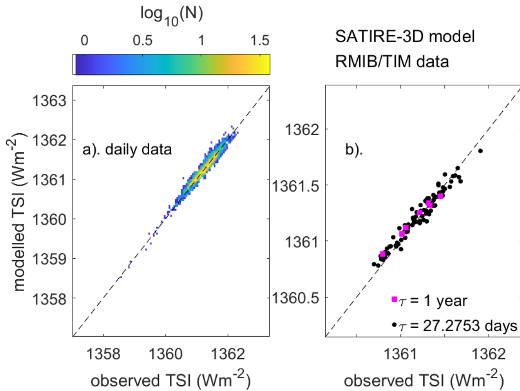
Figure 6. Scatter plots the SATIRE-3D model results with the TIM observations. (a) The logarithm of the number of daily samples in bins are 0.05 Wm^{-2} by 0.05 Wm^{-2} in extent, colour-coded as plotted a function of observed ( TSI_o ) and modelled ( TSI_m ) total solar irradiance. (b). Scatter plot of annual means of TSI_m as a function of TSI_o (mauve squares) over means over Carrington Rotation (CR) intervals (black dots). The dashed line show TSI_m = TSI_o .
