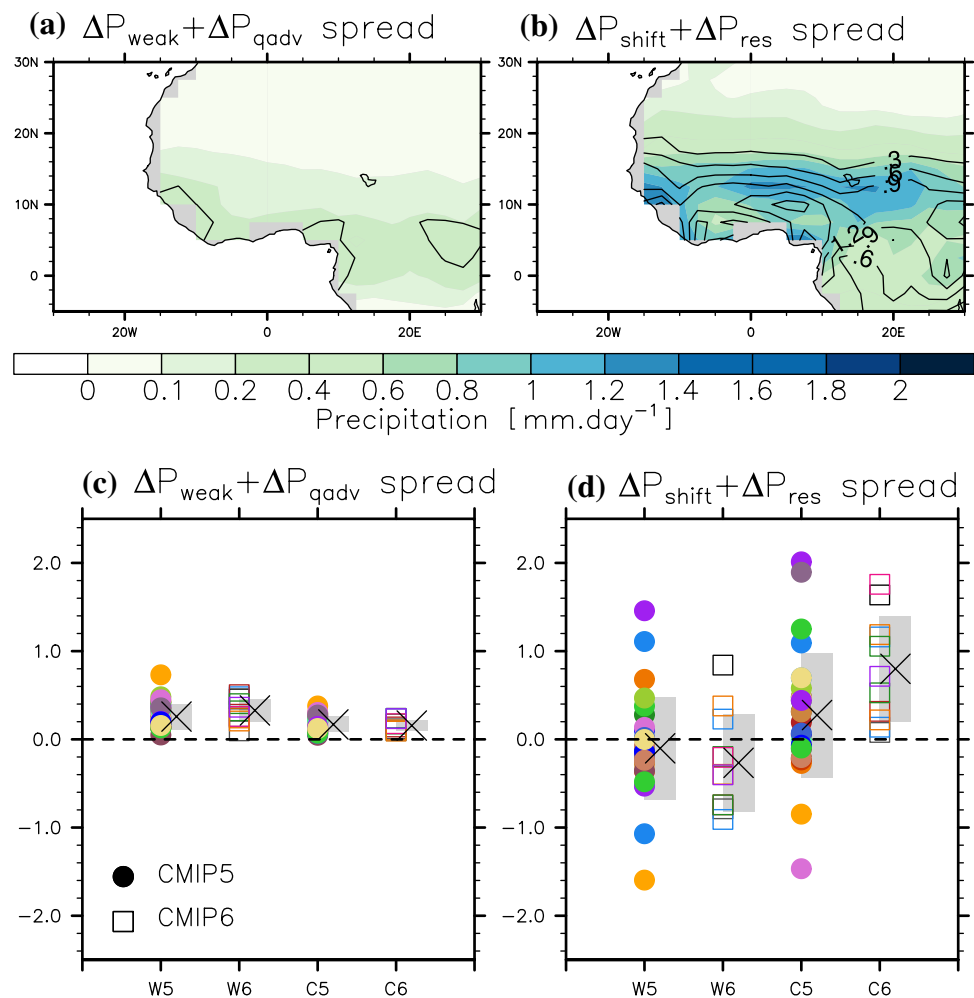
Fig. 5 Inter-model spread in a \Delta P_{\text{weak}} + \Delta P_{\text{qadv}} and b \Delta P_{\text{shift}} + \Delta P_{\text{res}} for the CMIP5 (colour) and the CMIP6 (black contours) ensemble. Changes in c \Delta P_{\text{weak}} + \Delta P_{\text{qadv}} and d \Delta P_{\text{shift}} + \Delta P_{\text{res}} for each model (colours), the multi-model mean average (black cross) and the inter-model spread (from one standard deviation; grey shading). CMIP5 simulations ("5") are represented by a filled circle while CMIP6 simulations ("6") are represented by an empty square. d–f Results are given for the western ("W") and the central ("C") Sahel. Please Fig. 2e for model's names
