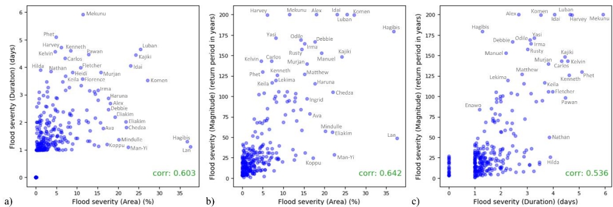
Figure 5: Scatter plots of the different flood severity indices: a) Flood severity (Area) vs Flood severity (Duration); b) Flood severity (Area) vs Flood severity (Magnitude); and c) Flood severity (Duration) vs Flood severity (Magnitude). The Spearman's Rank Correlation Coefficient is displayed on each plot. Points are annotated with the storm name if they have high values on either axis or are outliers to the general pattern.
