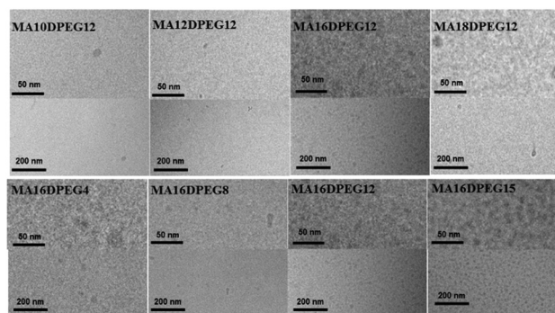
Fig. 1 Cryo-TEM images for the MAmDPEG n series (all 1 wt% aqueous solutions). For each sample, lower and higher magnification images are presented, to more clearly see the micelle structures.
