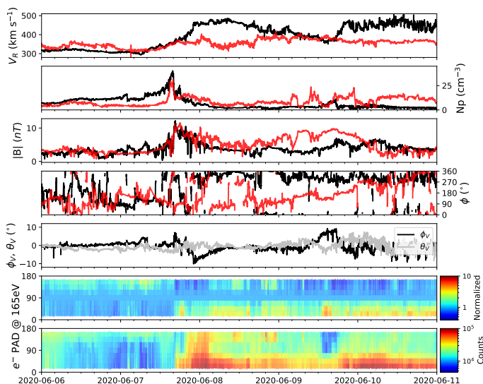
Fig. 3. The CIR observed by Wind and STEREO-A which represents the region O1 in Fig. 1. Here STEREO-A measurements (red), from the same source surface longitude, have been time shifted by \sim 6 days to line up with the increase in |B| . Wind observes a clear increase in solar wind speed from 300 \text{ km s}^{-1} to 465 \text{ km s}^{-1} , along with a distinctive east-west (positive-negative) deflection in the \phi_V signature. Both spacecraft observe a similar increase in |B| and N_p , but STEREO-A only measures an increase of 320 \text{ km s}^{-1} to 350 \text{ km s}^{-1} .
