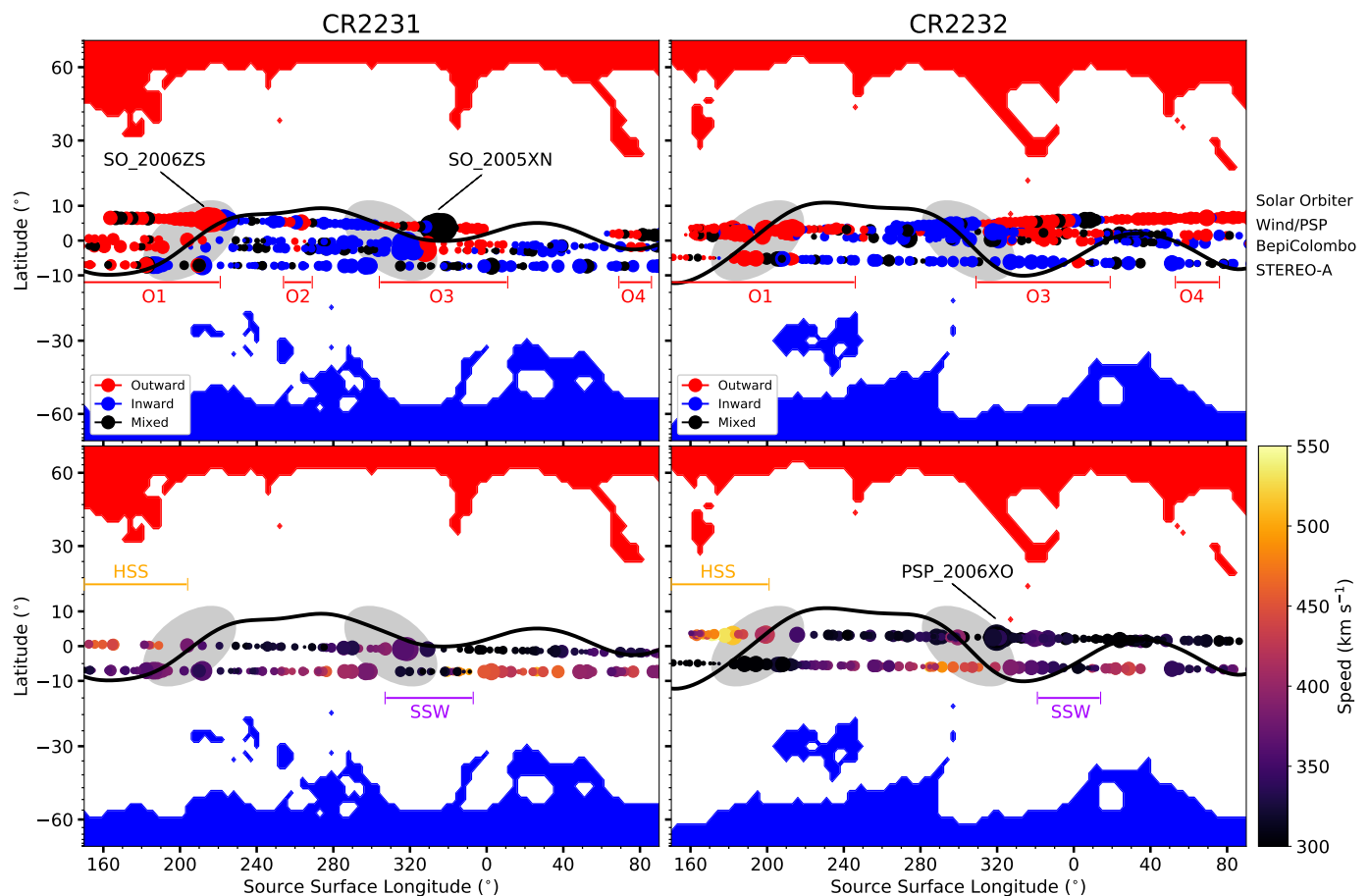
Fig. 1. Each scatter point represents a 6-hour average of the in situ parameters from a single spacecraft, where the size of the scatter point is proportional to (|B| \times R_{SC})^2 to accentuate changes in |B| . The top panels show the polarity measured by the different spacecraft for the two solar rotations, as outlined in Section 2, with the order of the spacecraft trails next to the top right panel. In these plots, each spacecraft travelled from right to left, where measurements of the same longitude were made by all the spacecraft within a few days, therefore minimising temporal effects. Open field lines are shown as the colourmap, as calculated from a PFSS model using an ADAPT magnetogram from the 1st June and 1st July for rotation CR2231 and CR2232, respectively. We ensured the output of the PFSS model was stable by considering the predicted HCS shape at daily intervals throughout the periods of interest, with the estimated HCS position shown as the solid black line, which broadly matches the shape of the in situ observations. The bottom left panel shows the solar wind speed from Wind (above) and STEREO-A (below), with the bottom right panel also displaying the data from PSP at the same latitude as Wind. These maps, along with the open field lines from PFSS, show that the CH structure was stable over the two rotations with a CIRs shown as highlighted grey regions at \sim 200^\circ and \sim 320^\circ longitude. This stable structure is also reflected in the polarity measurements, with outward polarity dips in the HCS outlined with the horizontal red lines. Transient structures are labelled with the according identification.
