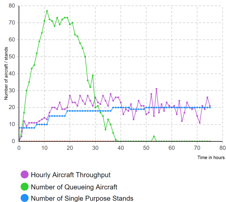
Figure 3. Hourly throughput of all aircraft, number of queueing aircraft recorded per hour, number of single purpose stands (y-axis - number of aircraft/stands, x-axis - time in hours)
