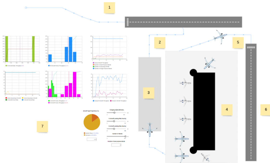
Figure 2 Simulation user interfaces showing an airport single pier model with a number of dual-purpose stands. Based on various pre-set parameters the DES model simulates aircraft arriving (1), taxiing to stand (2), queueing for a free stand (3), refuelling/recharging (4), then taxiing (5) to the runway for departure (6). Data (e. g. aircraft throughput) is then recorded and presented graphically on plots (7) as the simulation progresses.
