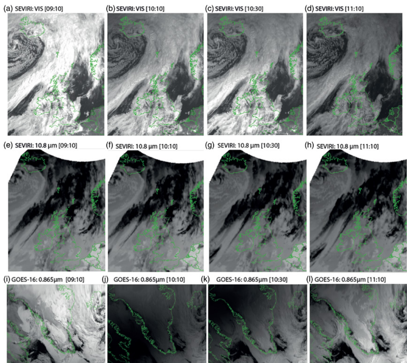
Figure 3. Satellite greyscale image sequences, showing cloud cover conditions during the eclipse period: (a–d) SEVIRI high-resolution visible broad bandwidth (0.6–0.9 μm) images and (e–h) SEVIRI Ch9 thermal infrared, for the British Isles/Iceland; panels (i–l) show GOES 16 CM-03 (0.865 μm) images of Greenland/Iceland. The eclipse shadow is evident in (j) and (k).
