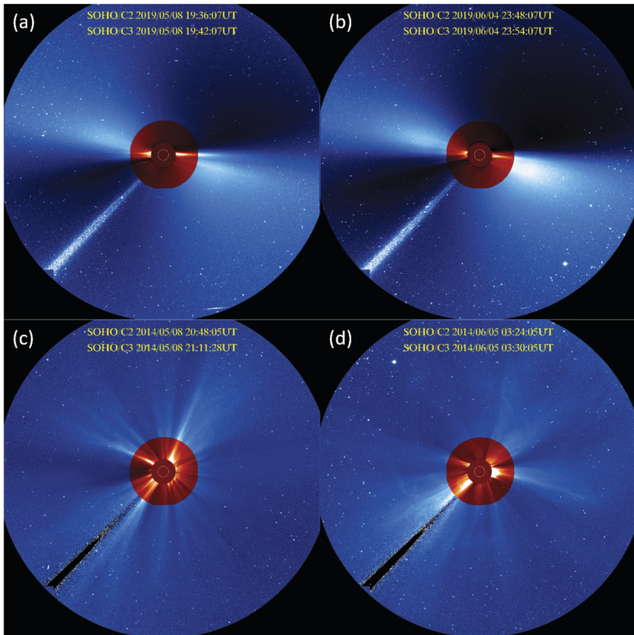
Figure 1 White-light images of the solar corona from the Large-angle Spectroscopic Coronagraph (LASCOCO) instrument on board the SOHO spacecraft. Panels a and b show images 27 days apart close to solar minimum, while panels c and d show images 27 days apart close to solar maximum.
