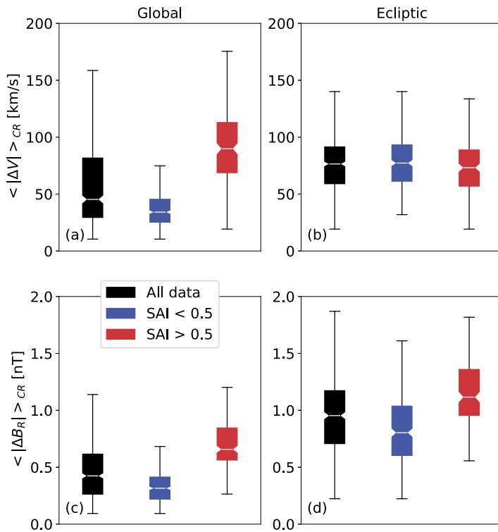
Figure 8 Box and whisker plots summarising the distributions of <|\Delta V|>_{CR} (panels a and b ) and <|\Delta B_R|>_{CR} (c and d ) obtained from consecutive solutions of HelioMAS at 1 AU. The white line shows the median, the coloured area spans with interquartile range (IQR), and the thin line spans the maximum to minimum values excluding outliers (i.e. 1.5 IQR above and below the third and first quartiles, respectively). The left-hand panels ( a and c ) show values averaged over all latitudes, the right-hand panels ( b and d ) show values at ecliptic latitudes (i.e. \pm 7.25^\circ about the solar equator). Black, blue, and red show all, low, and high solar-activity levels, respectively.)
