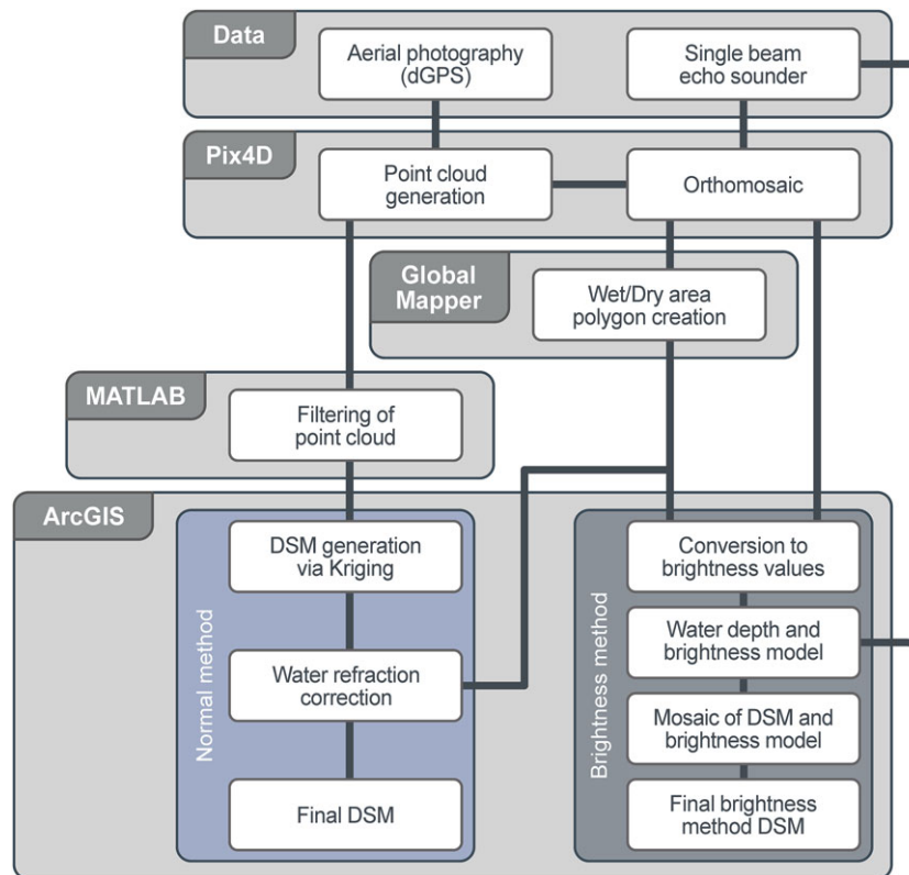
Figure 5. Workflow of DSM production from aerial images and the various data sources and computer programs employed. [Colour figure can be viewed at wileyonlinelibrary.com ] See the Terms and Conditions ( https://onlinelibrary.wiley.com/terms-and-conditions ) on Wiley Online Library for rules of use; OA articles are governed by the applicable Creative Commons License
