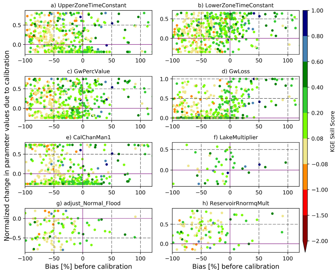
Fig. 9. The same as Fig. 8 but for mid-latitude basins (with a significant negative bias in the baseline streamflow).
