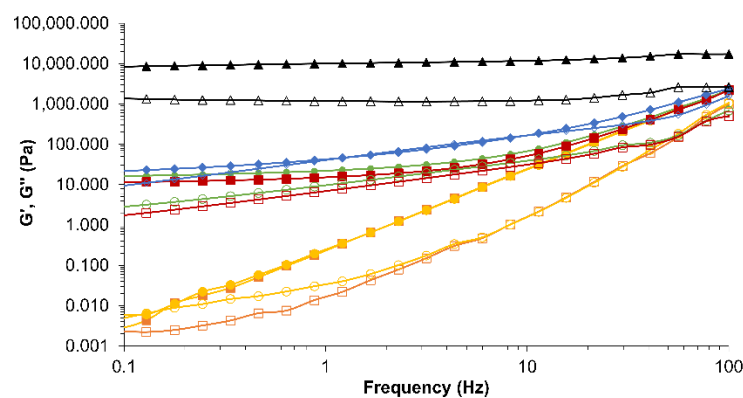
Figure 4. Dynamic moduli as a function of frequency of emulsions and butter ▲. Conventional emulsion (CE-0 ■; CE-2 ■; CE-4 ◆). Nanoemulsion (NE-0 ●; NE-2 ●). Filled symbols correspond to elastic modulus ( G' ) and open symbols to viscous modulus ( G'' ).
