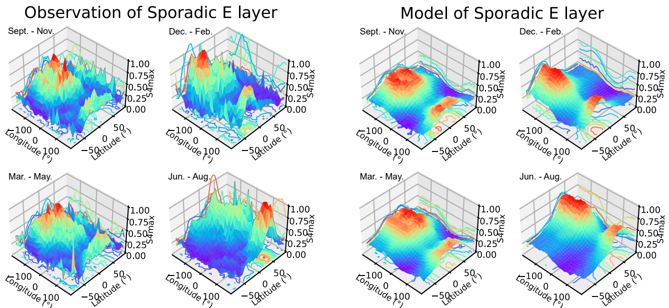
Figure 10. Global distributions of the intensity of E_s layers at 0 UT in the four seasons, represented by S4max from satellite radio occultation observations and the model outputs in the period 2006–2014. Plots for the autumn (September, October, and November) in the top left, the winter (December, January, and February) in the top right, the spring (March, April, and May) in the bottom left, and the summer (June, July, and August) in the bottom right.
