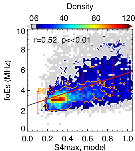
Figure 12. Density scatter plot of the hourly manually scaled f_oE_s measured by an ionosonde at Beijing versus the hourly S4max model outputs in the period 2006–2014. The orange and white contour lines represent 50% and 90% of the number of data. The red line represents the linear least-squares fit with the standard deviation from the mean within a 0.15 S4max band.
