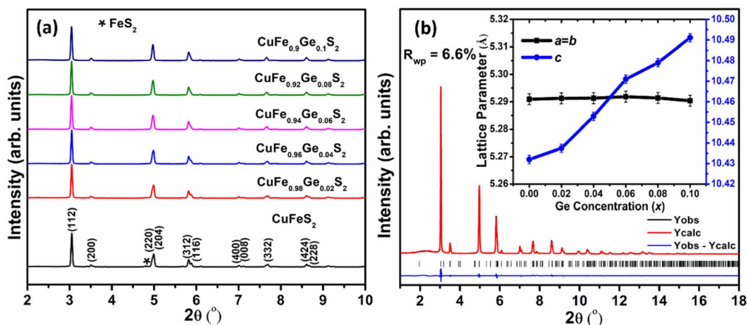
Fig. 2 (a) Synchrotron X-ray powder diffraction patterns ( \lambda = 0.161669 \text{ Å} ) collected for CuFe 1-x Ge x S 2 ( 0.0 \leq x \leq 0.10 ). (b) Rietveld refinement using powder X-ray diffraction data for CuFe 0.94 Ge 0.06 S 2 . The inset shows the lattice parameters as a function of Ge content ( x ).
