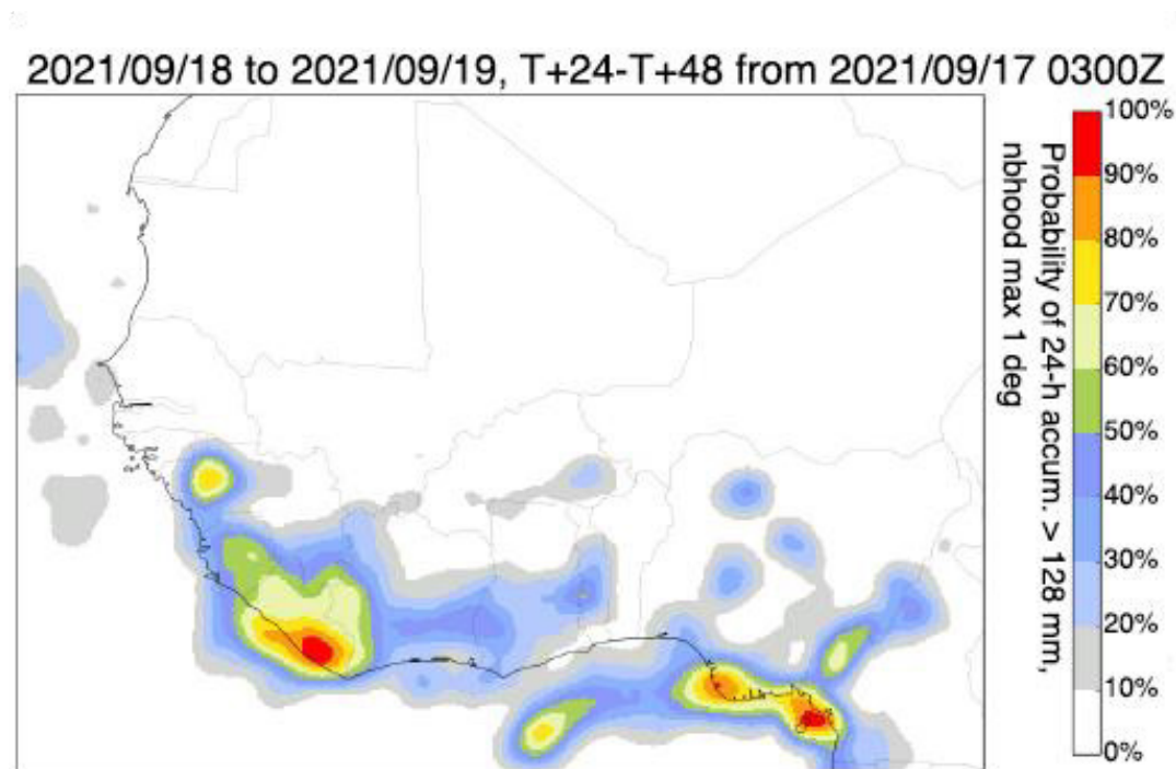
Fig. 4: Example of a convection-permitting ensemble product provided to forecasters during the testbed. Neighborhood method is described in Cafaro et al (2021) following Roberts and Lean (2008).
