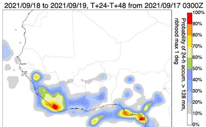
Fig. 4. Example of a convection-permitting ensemble product provided to forecasters during the testbed. The neighborhood method is described in Cafaro et al. (2021) following Roberts and Lean (2008).
