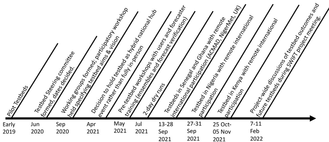
Fig. 1. (a) Example probability of rainfall accumulation map from the Met Office regional convection-permitting ensemble forecast system, with the locations of the African testbed participants indicated by red stars. (b) Timeline of testbed preparation and delivery (see appendix D for details on testbed preparation).
