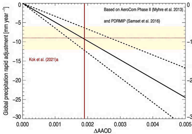
Fig. 12. A lower bound on the inhibition of global mean precipitation by dust-induced absorption. The black lines show the overall relationship between AAO and precipitation reduction from rapid adjustments derived from multi-model studies, and the black dashed lines show the range of uncertainty. The red line shows the estimate of total dust SW AAO shown in Fig. 9 based on (Kok et al., 2021a) and the resulting constraint (yellow shading).
