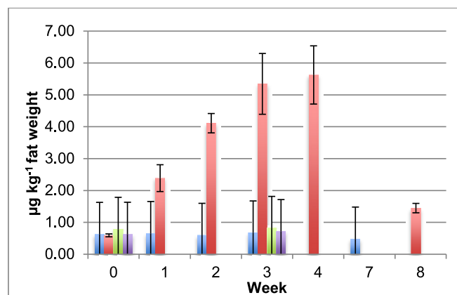
Fig. 2. Upper bound \Sigma ICES 6 PCB concentrations in milk (fat weight basis) for cattle ingesting diets amended with the following treatments: ■, Control (soil), ■, Biosolids, ■, Biosolids-soil and ■, CLO-soil; Where values were < LoQ the LoQ was used to calculate the mean; Error bars show the standard deviation of the mean.
