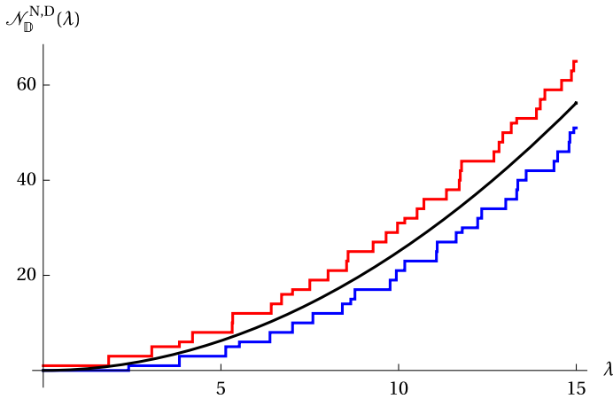
Fig. 1 The Dirichlet eigenvalue counting function \mathcal{N}_{\mathbb{D}}^{\mathbb{D}}(\lambda) (blue), the Neumann eigenvalue counting function \mathcal{N}_{\mathbb{D}}^{\mathbb{N}}(\lambda) (red), and the leading Weyl's term W_d(\lambda) = \frac{\lambda^2}{4} (black) in dimension d = 2 . The plot is produced using the floating-point evaluation of zeros of the Bessel functions and their derivatives. If we were to assume (contrary to the philosophy of this paper) the validity of floating-point arithmetic, this plot would have presented a numerically assisted (as opposed to computer-assisted ) “proof” of Pólya's conjecture for the disk for \lambda \lesssim 15
