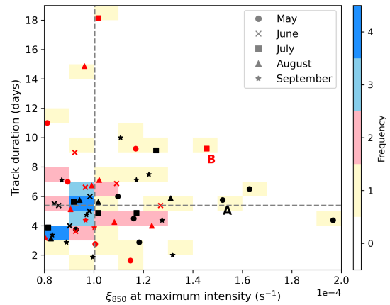
Figure 1. The 2-D histogram of \xi_{850} at maximum intensity ( x axis) and track duration ( y axis) of summer 2020 Arctic cyclones from ERA5. Black and red markers refer to low-level and upper-level-dominant cyclones respectively, as diagnosed by the thermal Rossby number, Ro_T , from the modified cyclone phase space (Sect. 2.4) at the time of maximum growth rate. The shading illustrates the number of cyclones that populate a region of the histogram space. The median values of \xi_{850} at maximum intensity and track duration are demonstrated by the dashed grey lines. Cyclone cases A and B are annotated with the respective letter to the bottom right of the marker.
