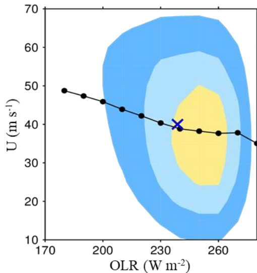
Fig.9 Joint pdfs of daily OLR (abscissa) and 3-day lagged U_{200-250} at 30^{\circ}\text{S} (ordinate), for the Latitude Circle (LC). The black dots joined by a line indicate the average value of U for each OLR bin. The other conventions and details are as in Fig.5.
