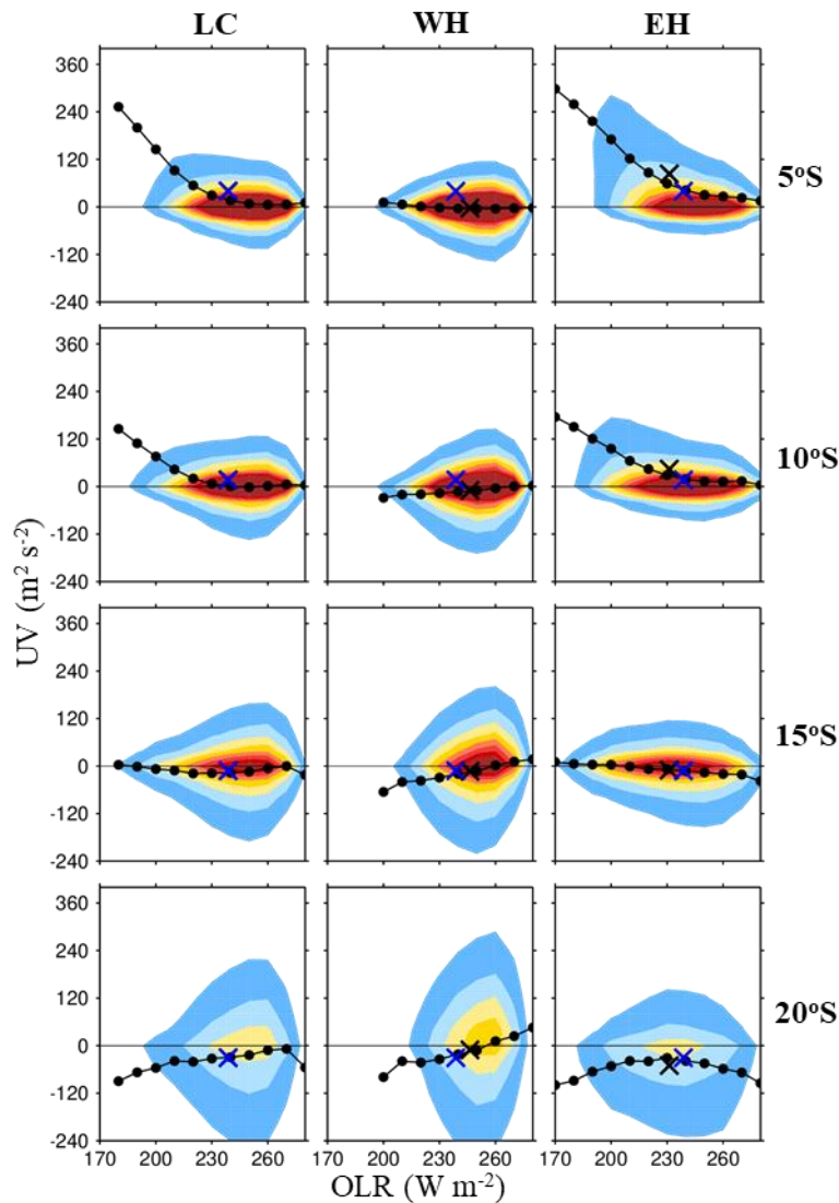
Fig. 6. Joint pdfs of daily OLR (abscissa) and total northward flux of westerly momentum, UV (ordinate). The columns are for the Latitude Circle (LC), the Western Hemisphere (WH), and the Eastern Hemisphere (EH), and the rows are for 5°S, 10°S, 15°S, 20°S. The conventions and details are as in Fig.5.
