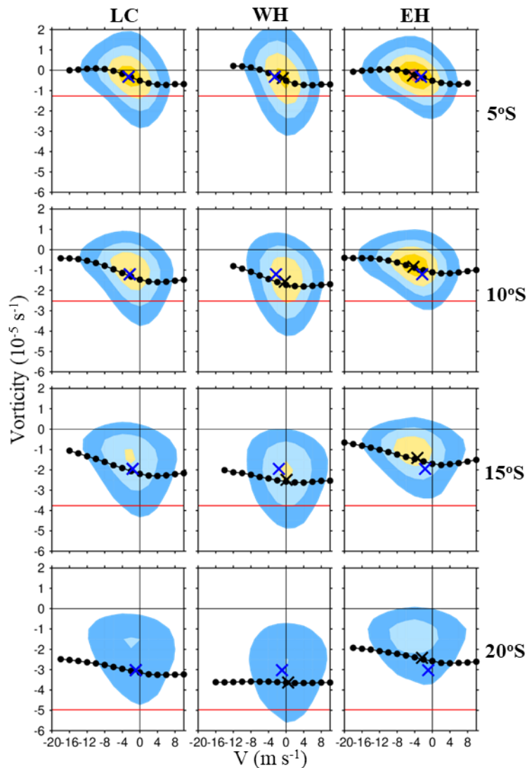
Fig. 8. Joint pdfs of daily V (abscissa) and absolute vorticity, \zeta (ordinate). The columns are for the Latitude Circle (LC), the Western Hemisphere (WH) and the Eastern Hemisphere (EH), and the rows are for 5^{\circ}\text{S} , 10^{\circ}\text{S} , 15^{\circ}\text{S} , 20^{\circ}\text{S} . The data for the two variables is taken from the values at the same grid-point and time. The black dots joined by a line indicate the average value of \zeta for each V bin. In each panel, the horizontal red
