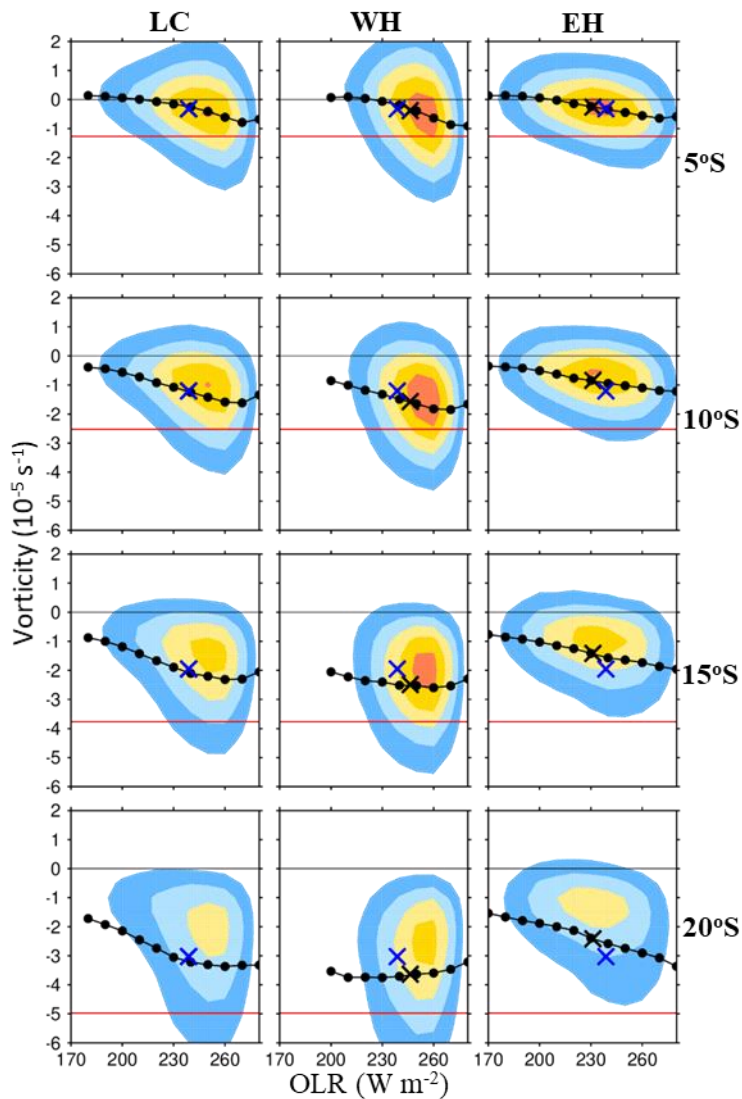
Fig. 7. Joint pdfs of daily OLR (abscissa) and absolute vorticity, \zeta (ordinate). The columns are for the Latitude Circle (LC), the Western Hemisphere (WH) and the Eastern Hemisphere (EH), and the rows are for 5°S, 10°S, 15°S, 20°S. The horizontal red lines in each panel indicate the value of the Coriolis parameter at the central latitude. The conventions and details are as in Fig.5.
