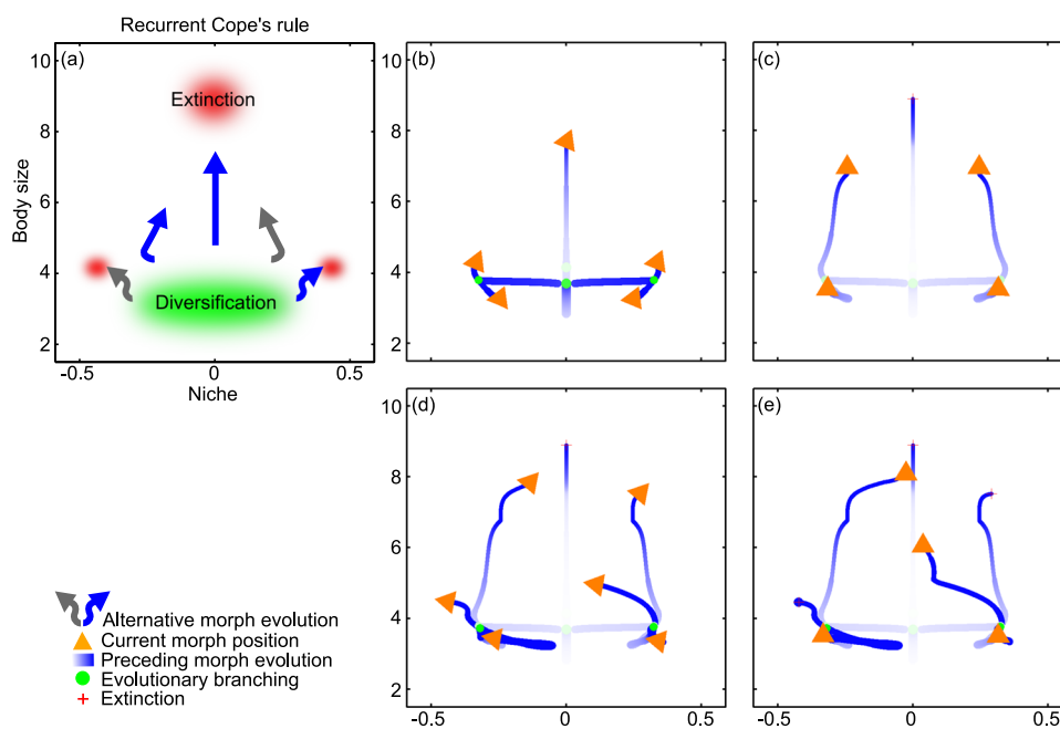
Fig. 3 Evolution in body size and niche with precarious top predators: recurrent Cope's rule. a Schematic illustration of phylogenetic pattern. b–e Trait combinations in the coevolving community at four successive times. Orange arrowheads show species' current trait values and the current directions of the selection pressures governing their evolutionary change. Blue motion trails represent species' evolutionary trajectories, with their thickness being proportional to species' population densities and with the darkest blue corresponding to the current time. Green circles and red crosses, respectively, indicate past trait combinations at which evolutionary diversifications and species extinctions occurred. In this macroevolutionary pattern, evolutionary diversification occurs at small body sizes: all species then evolve toward larger body sizes, punctuated by the recurrent extinction of top predators. For a dynamic rendering of the shown community coevolution, see Supplementary Movie S3. For a full dynamical rendering of the shown community coevolution, see Supplementary Movie S3. Parameters as shown in Table 1, with \alpha = 0.002 and e = 0.005 .
